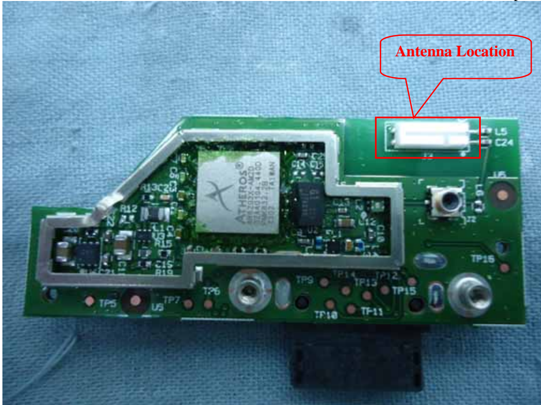
Figure 4 Wireless Module (Component Side)
