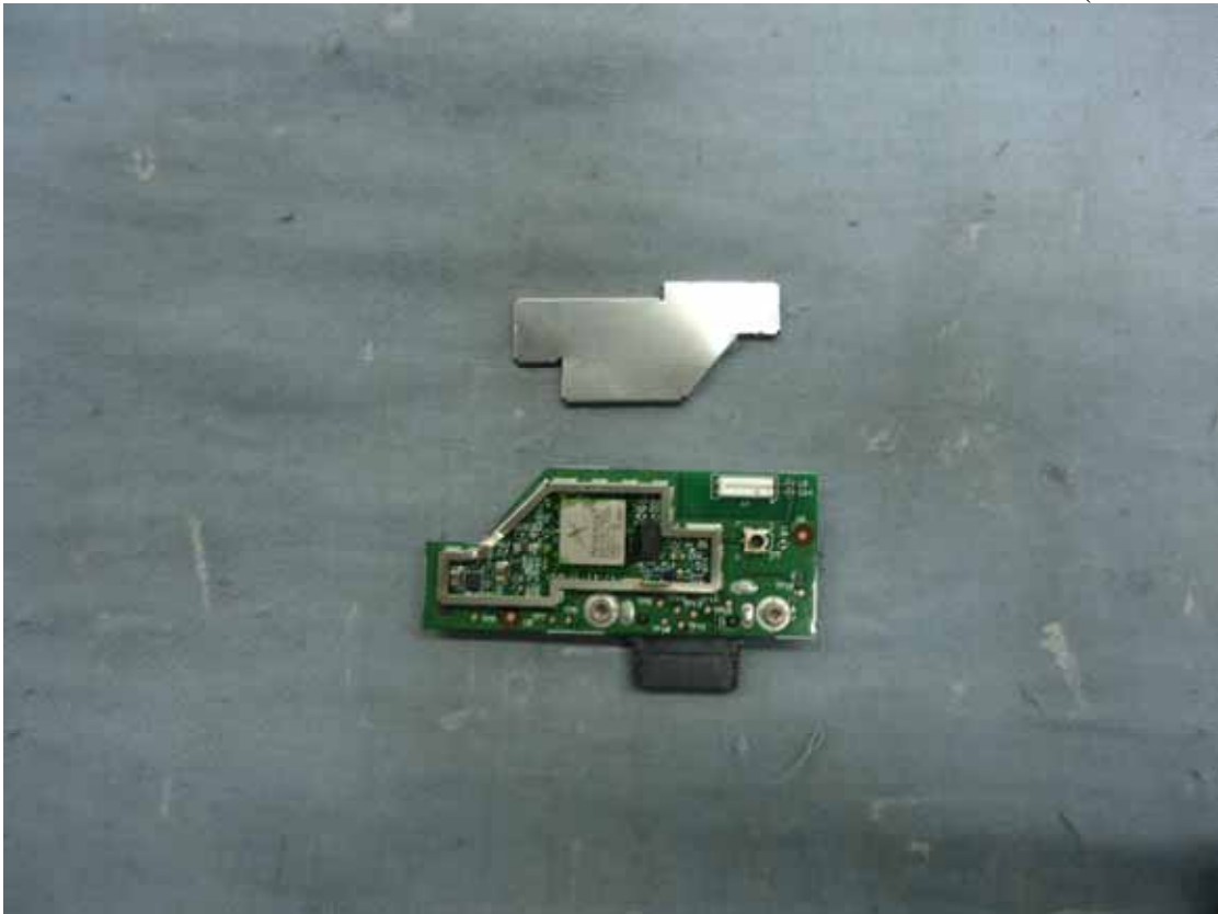
Figure 3 Wireless Module (Cover Removed)
