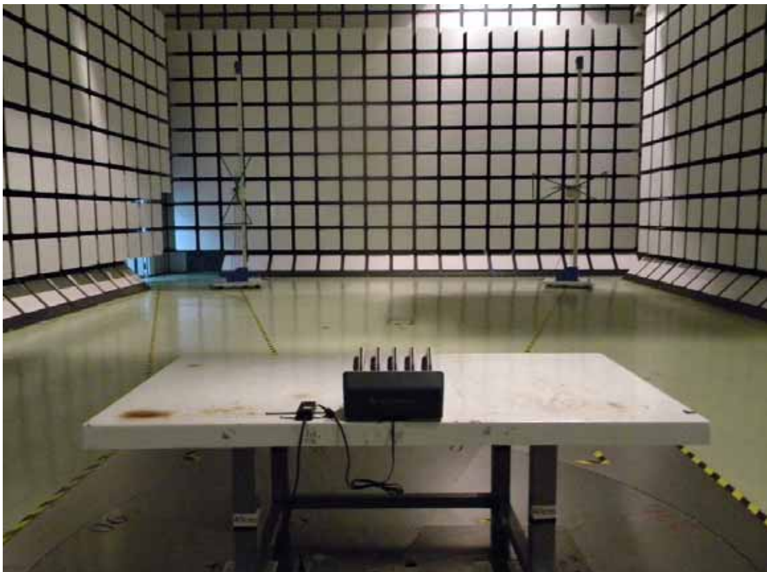
Back View of Radiated Measurement (Configuration B)
