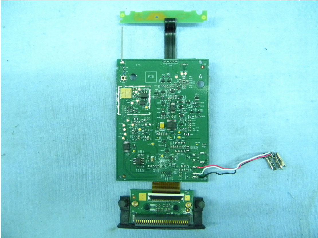
Figure 6 PCB Board (Solder Side)
