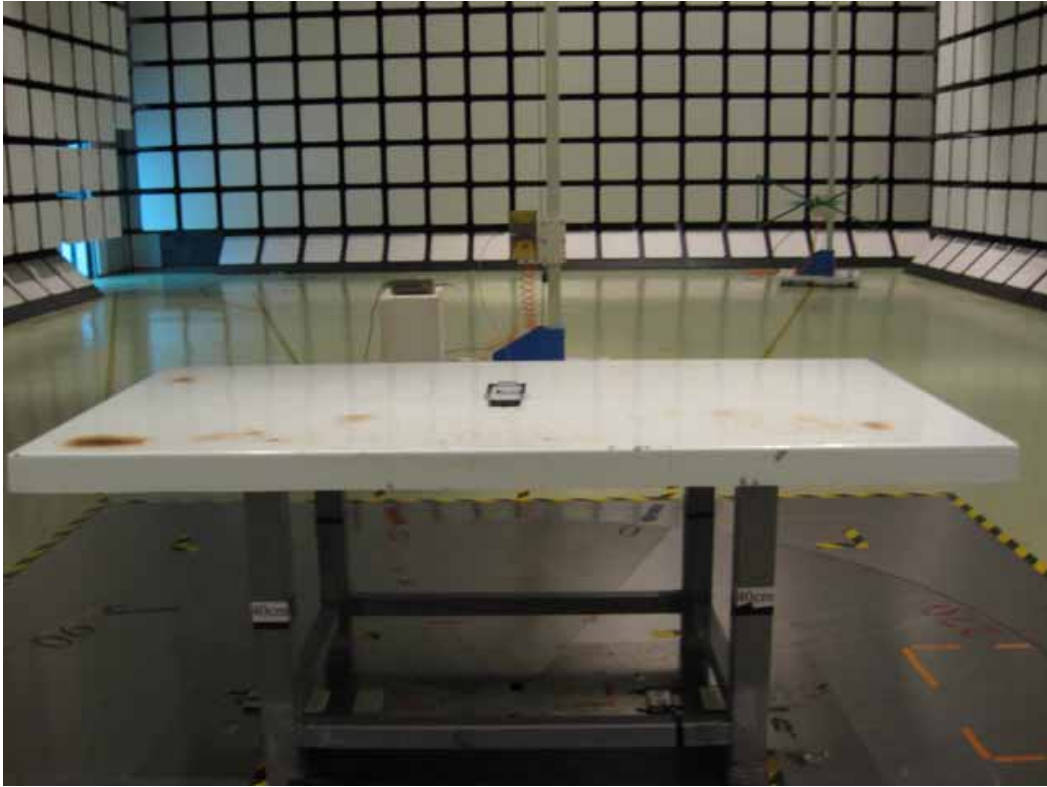
Front View of Radiated Disturbance Measurement
