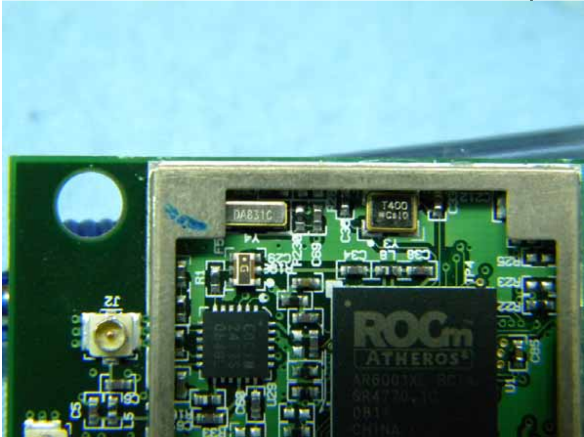
Figure 9 Crystal Oscillator
