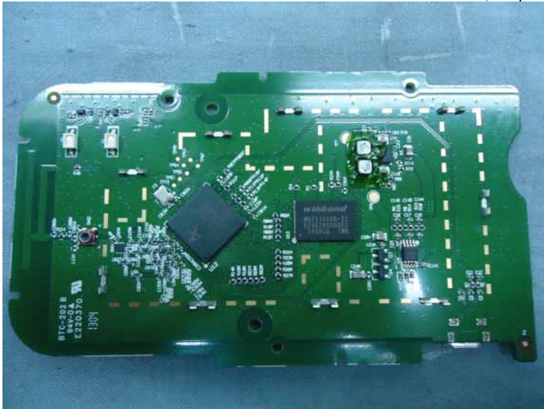
Figure 5 Wireless Module (Component Side)
