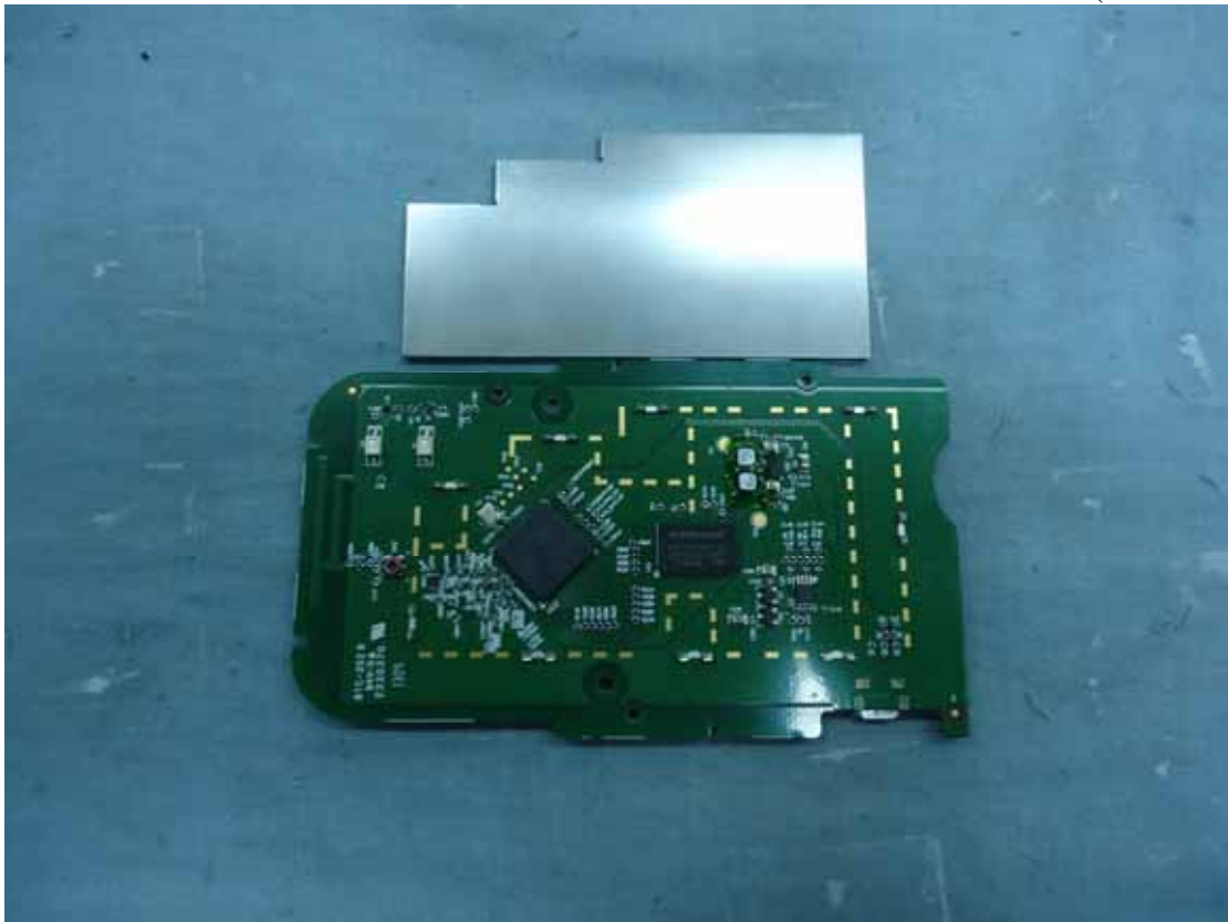
Figure 4 Wireless Module (Cover Removed)
