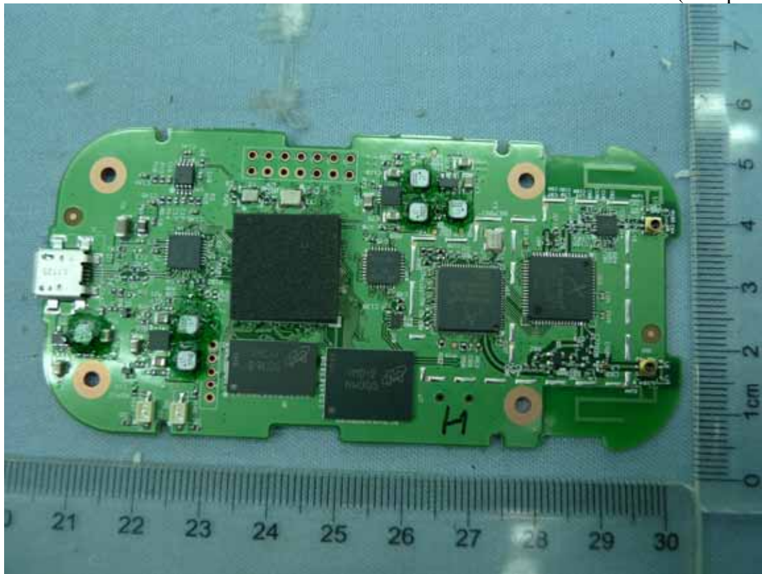
Figure 3 Wireless Module (Component Side)
