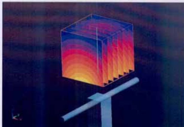
0 dB = 16.830mW/g
