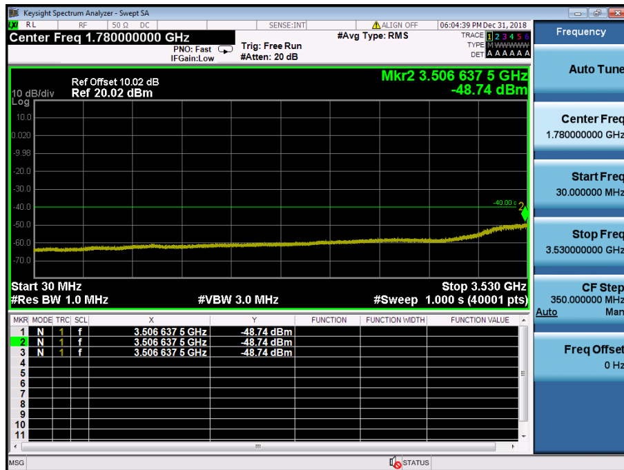
LTE Band 48 / 15 MHz / QPSK - RB Size/Offset (75/0) – High Channel_1
