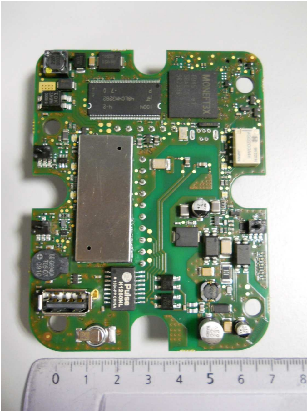
IntPho-2 : Front side of electronic board with shield cover
