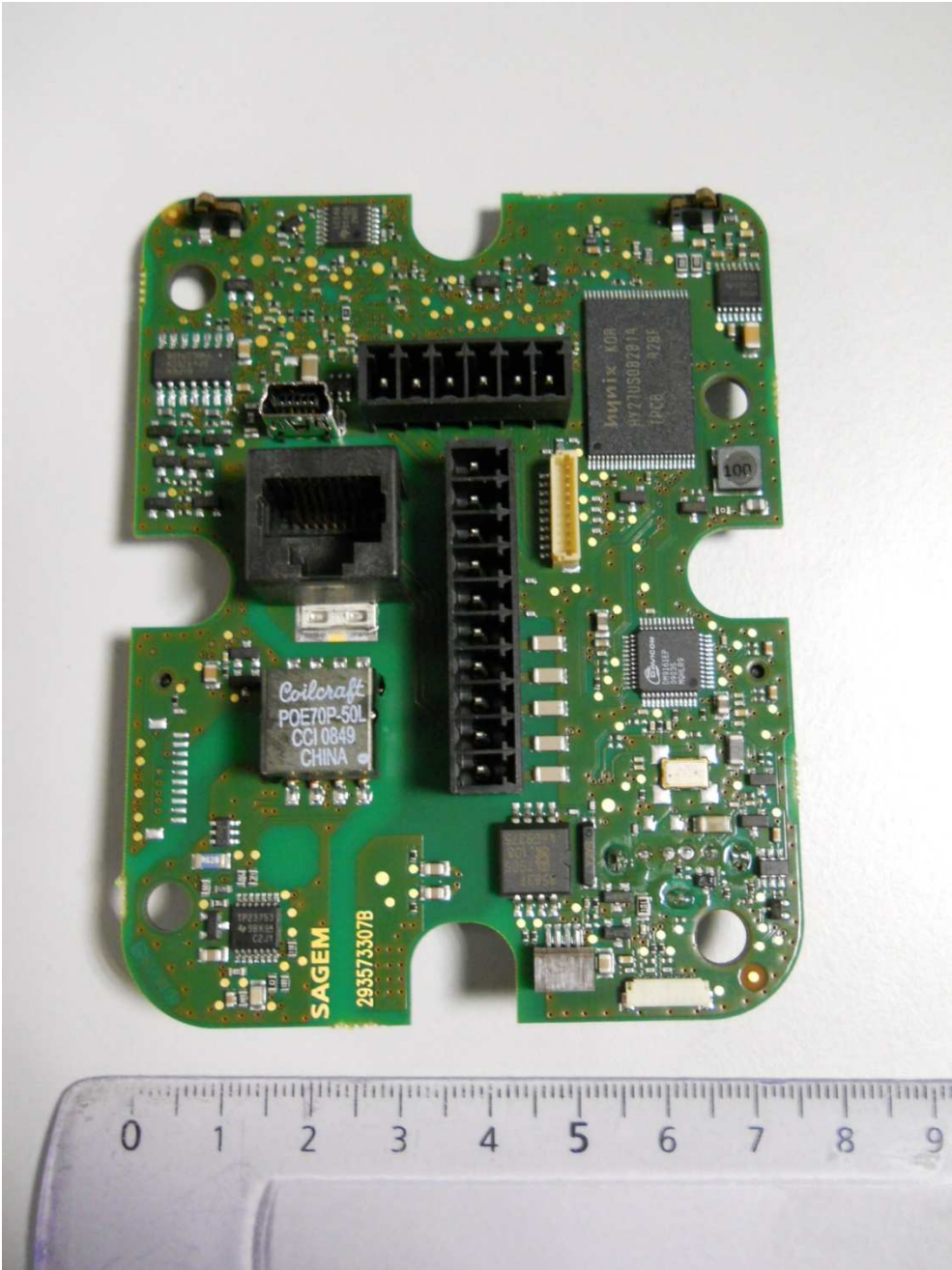
IntPho-3 : Rear side of electronic board
