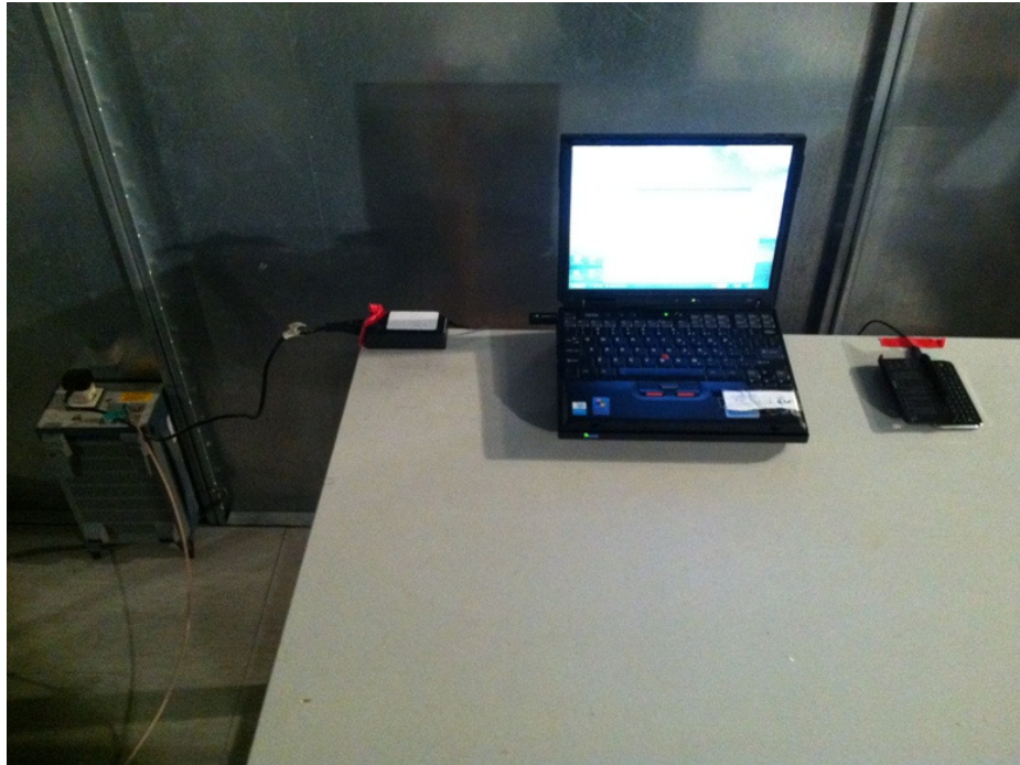
Set-up for AC wire line conducted emissions
