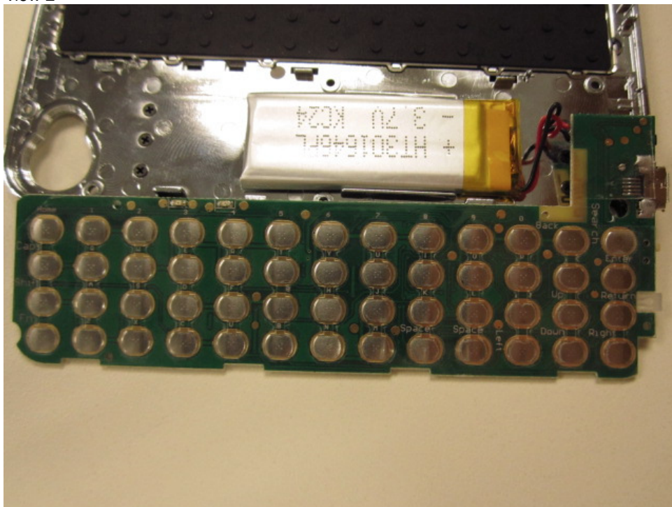
1.1.10 Side view 2
