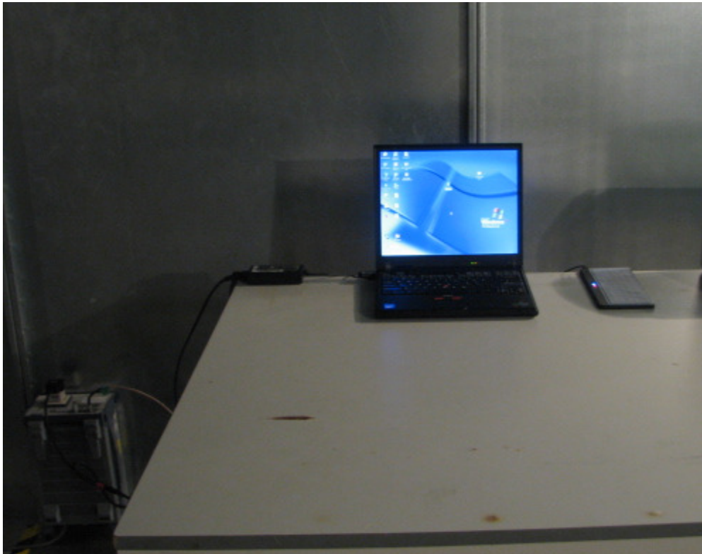
Set-up for AC wire line conducted emissions
