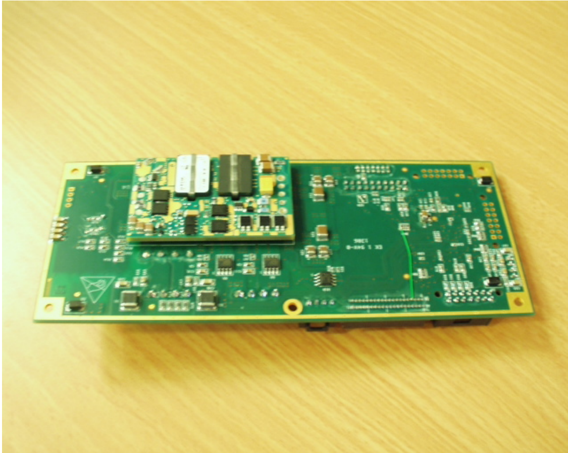
Picture 14: PSC card (power supply card) bottom side
