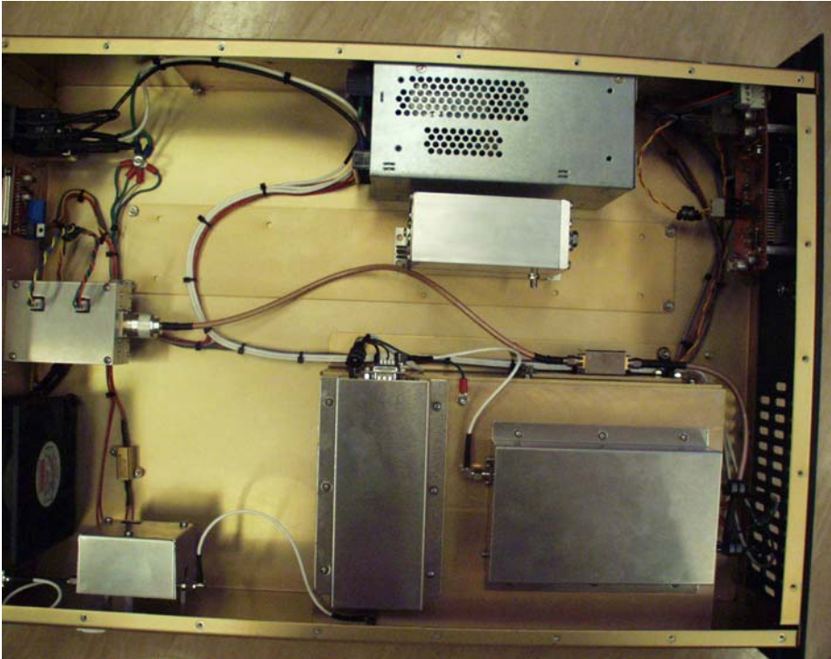
Picture 2: PA internal view (final stage at lower right side)
