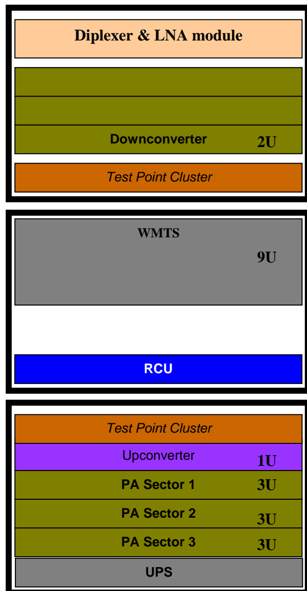
Figure 1: Rack Layout diagram
