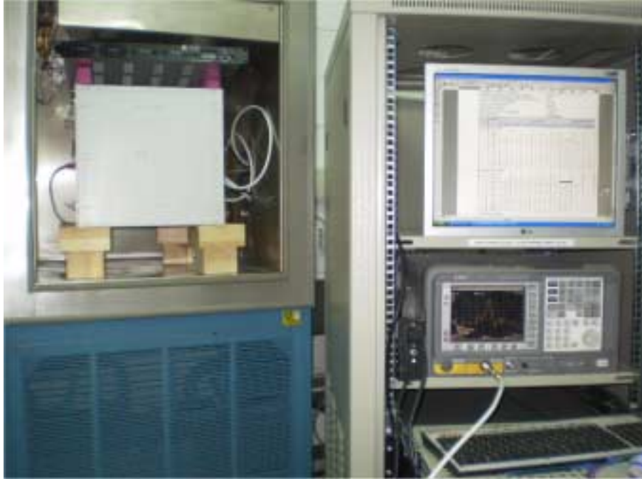
Photograph No.8 Setup for frequency stability measurements
