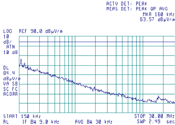
Plot 7.6.4 Radiated emission measurements in 0.15 - 30 MHz range
