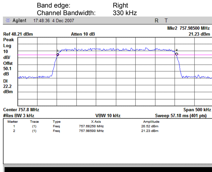
Plot 7.8.8 Band edge emission at high frequency, 256QAM
