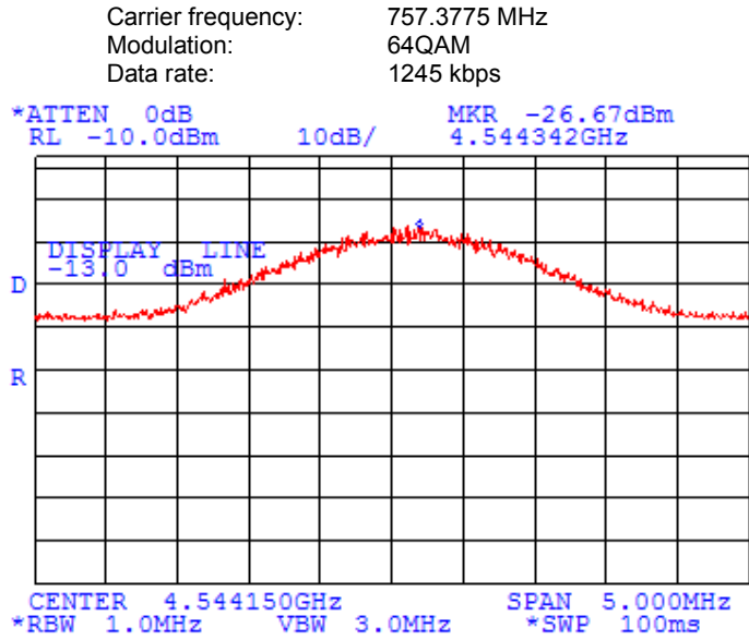
Plot 7.3.17 Spurious emission measurements at RF antenna connector, the 6 th harmonic of the mid channel
