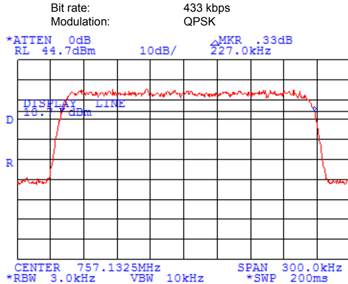
Plot 7.9.1 Occupied bandwidth test results at low frequency
