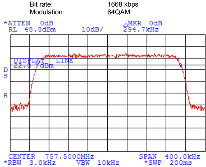
Plot 7.9.19 Occupied bandwidth test results at mid frequency
