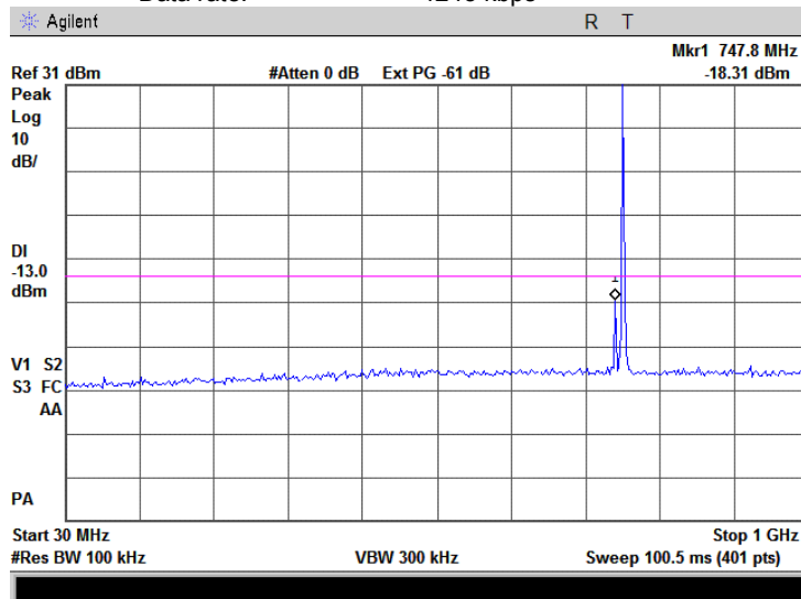
Plot 7.3.8 Spurious emission measurements at RF antenna connector, mid channel
