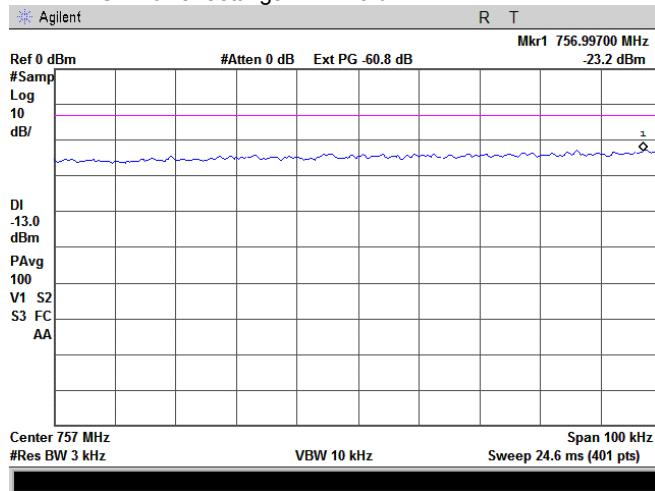
Plot 7.5.32 emissions at RF antenna connector, low channel band edge measurements
