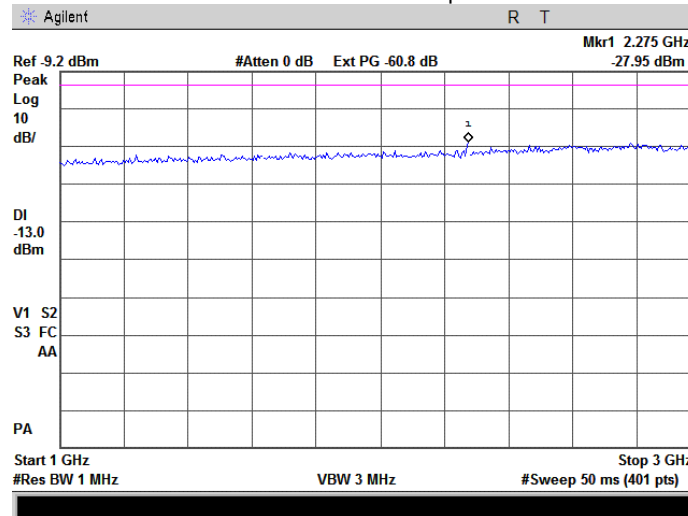
Plot 7.3.30 Spurious emission measurements at RF antenna connector, high channel
