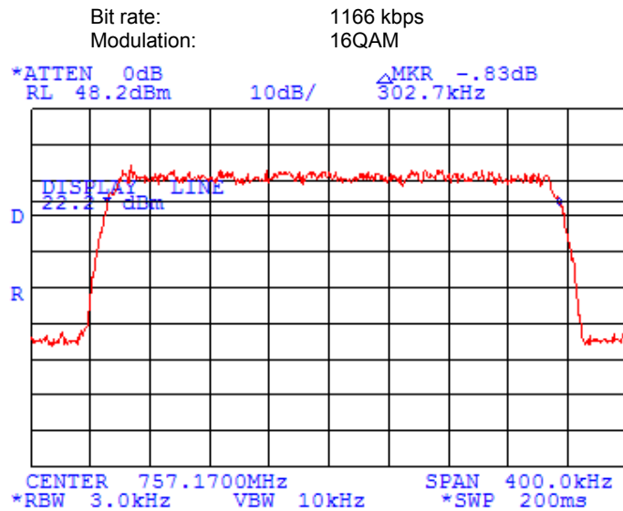
Plot 7.9.14 Occupied bandwidth test results at low frequency
