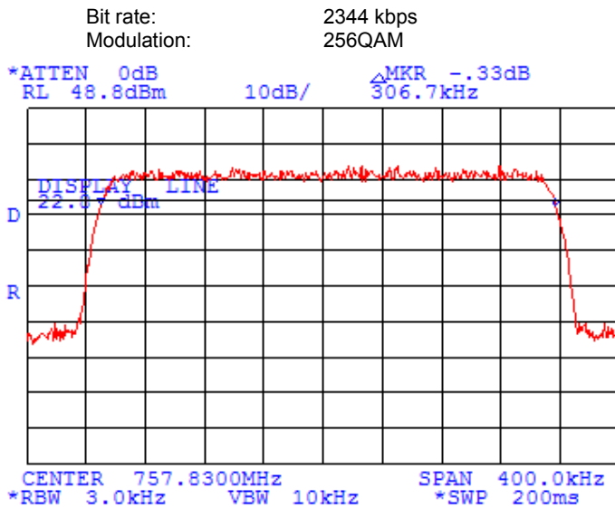
Plot 7.9.24 Occupied bandwidth test results at high frequency
