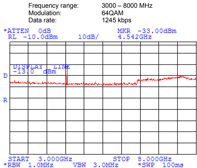
Plot 7.3.14 Spurious emission measurements at RF antenna connector, mid channel
