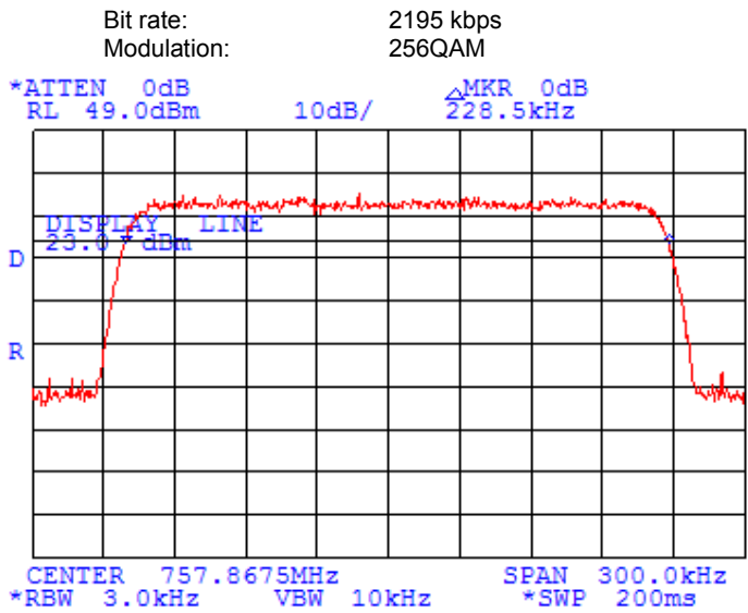
Plot 7.9.12 Occupied bandwidth test results at high frequency
