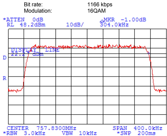
Plot 7.9.22 Occupied bandwidth test results at high frequency
