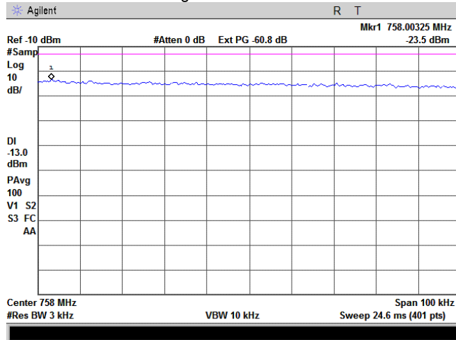
Plot 7.5.47 Spurious emissions at RF antenna connector, high channel band edge measurements
