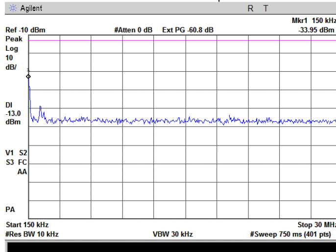
Plot 7.3.24 Spurious emission measurements at RF antenna connector, high channel
