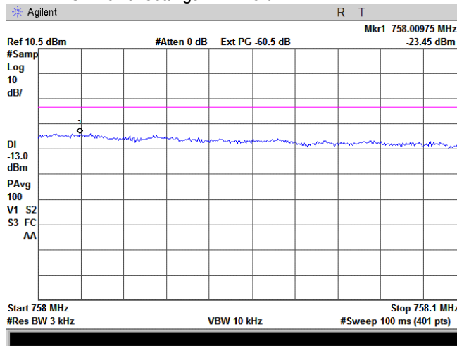
Plot 1.7.5.5 Spurious emissions at RF antenna connector, high channel band edge measurements
