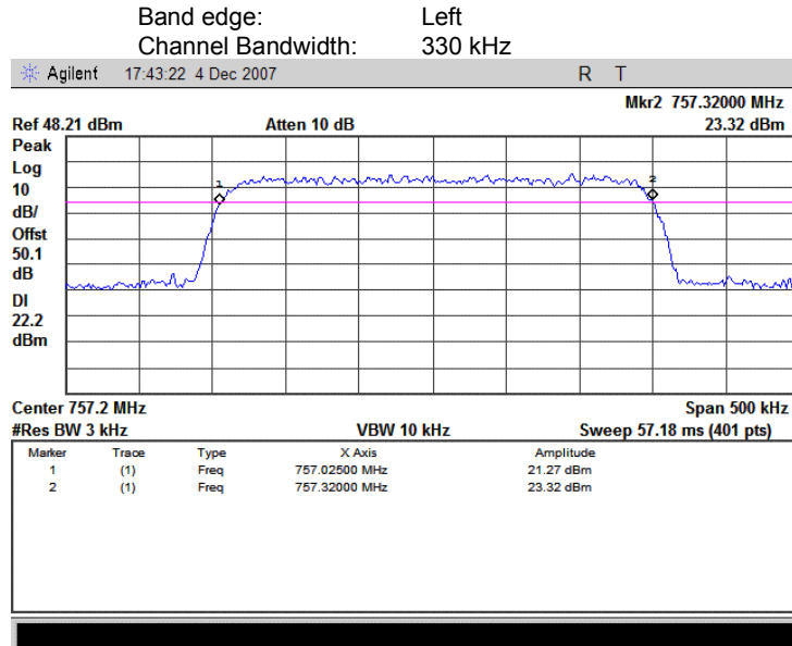
Plot 7.8.4 Band edge emission at low frequency, 256QAM
