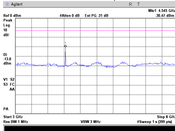
Plot 7.3.32 Spurious emission measurements at RF antenna connector, mid channel
