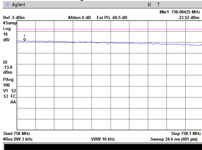
Plot 7.5.17 Spurious emissions at RF antenna connector, high channel band edge measurements
