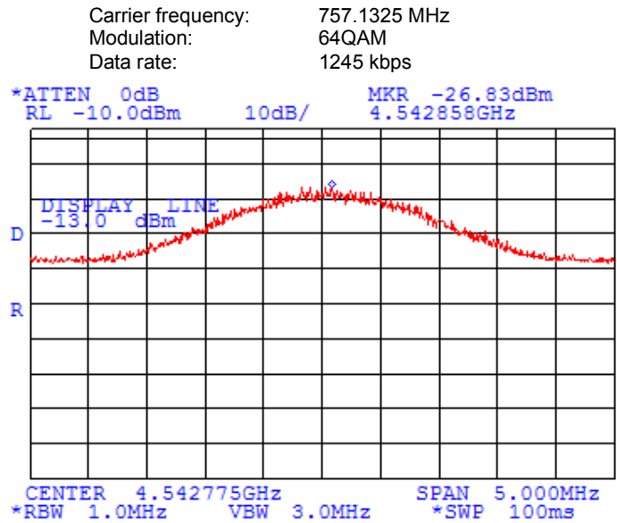
Plot 7.3.16 Spurious emission measurements at RF antenna connector, the 6 th harmonic of the low channel
