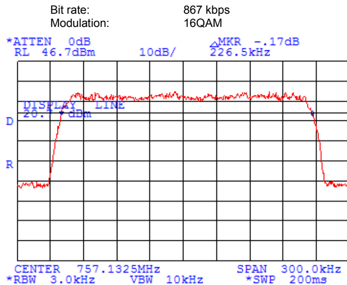
Plot 7.9.2 Occupied bandwidth test results at low frequency
