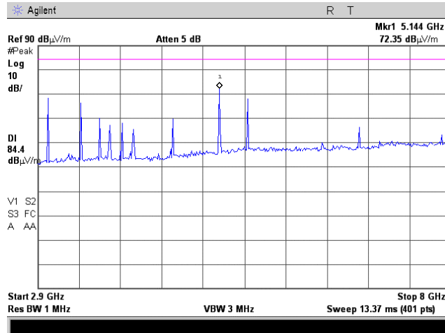
Plot 7.6.10 Radiated emission measurements in 2.9 – 8.0 GHz range
