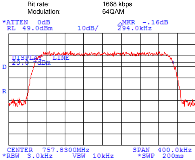
Plot 7.9.23 Occupied bandwidth test results at high frequency
