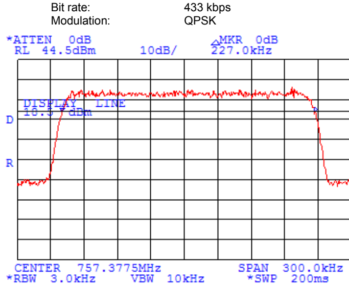
Plot 7.9.5 Occupied bandwidth test results at mid frequency
