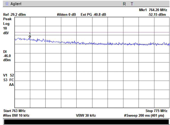
Plot 7.4.10 Spurious emission test results at high frequency
