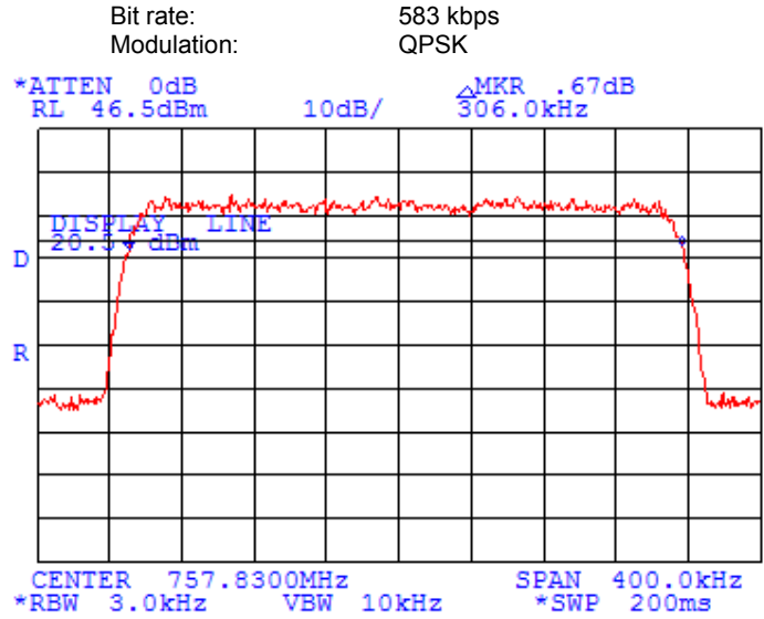
Plot 7.9.21 Occupied bandwidth test results at high frequency
