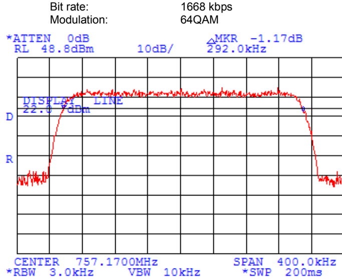
Plot 7.9.15 Occupied bandwidth test results at low frequency
