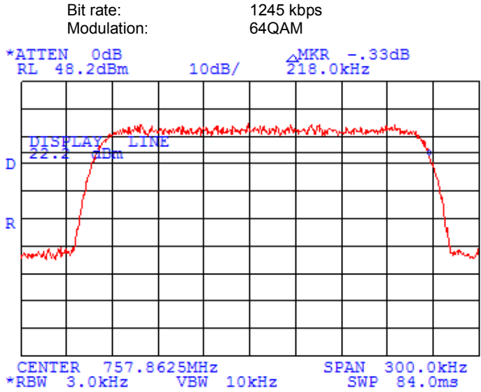
Plot 7.9.11 Occupied bandwidth test results at high frequency
