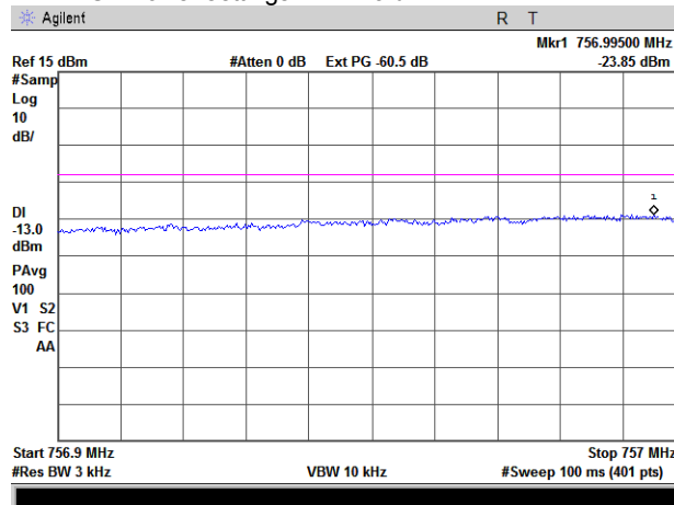
Plot 7.5.8 Spurious emissions at RF antenna connector, low channel band edge measurements
