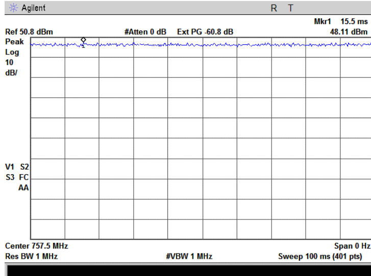
Plot 7.1.1 Duty cycle measurement
