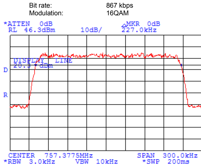
Plot 7.9.6 Occupied bandwidth test results at mid frequency
