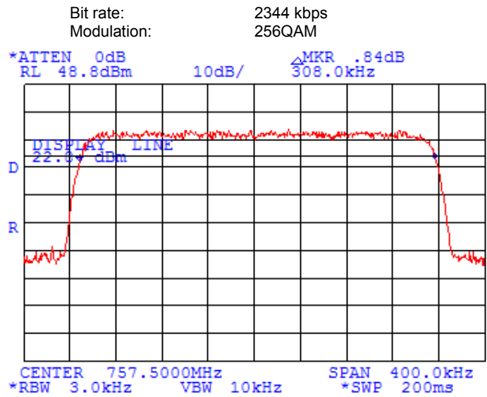
Plot 7.9.20 Occupied bandwidth test results at mid frequency
