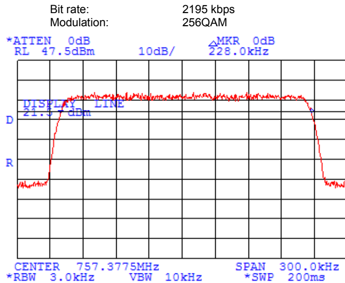
Plot 7.9.8 Occupied bandwidth test results at mid frequency
