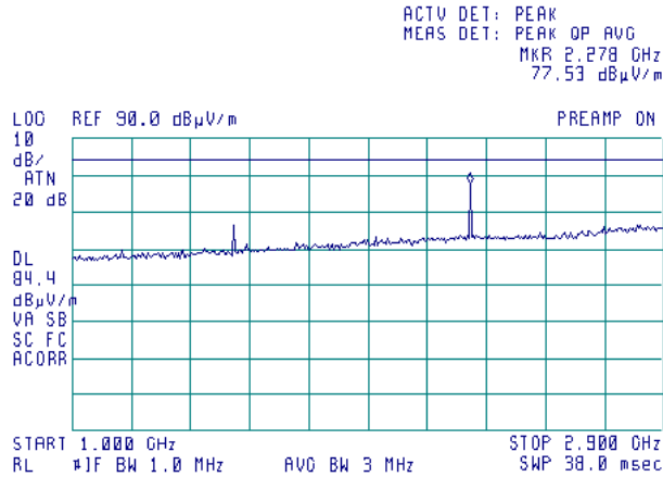
Plot 7.6.8 Radiated emission measurements in 1 – 2.9 GHz range
