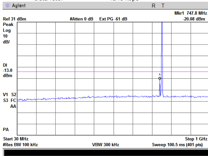
Plot 7.3.10 Spurious emission measurements at RF antenna connector, low channel
