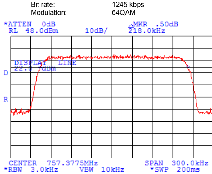
Plot 7.9.7 Occupied bandwidth test results at mid frequency
