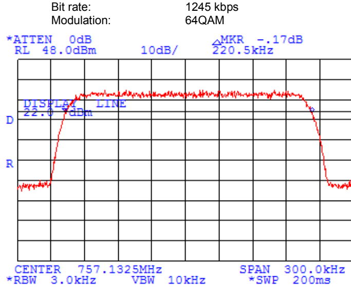
Plot 7.9.3 Occupied bandwidth test results at low frequency
