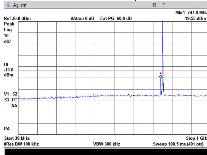
Plot 7.3.26 Spurious emission measurements at RF antenna connector, mid channel
