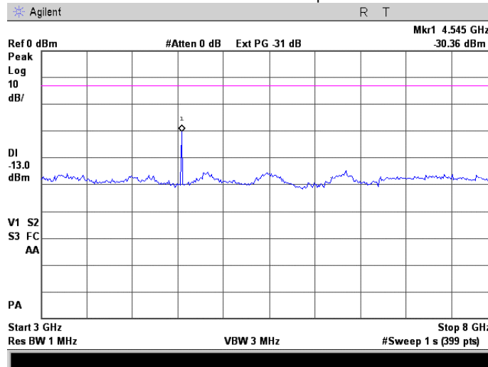
Plot 7.3.34 Spurious emission measurements at RF antenna connector, the 6 th harmonic of the low channel
