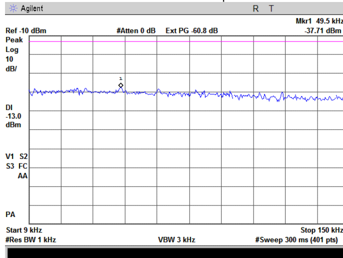
Plot 7.3.22 Spurious emission measurements at RF antenna connector, low channel
