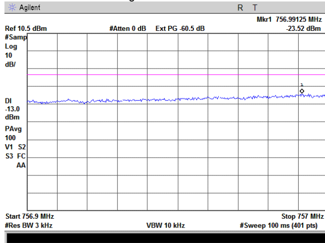
Plot 7.5.2 Spurious emissions at RF antenna connector, low channel band edge measurements
