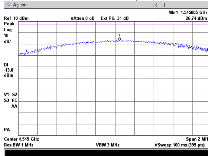
Plot 7.3.36 Spurious emission measurements at RF antenna connector, the 6 th harmonic of the High channel
