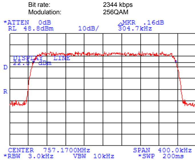
Plot 7.9.16 Occupied bandwidth test results at low frequency
