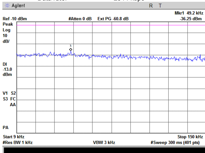
Plot 7.3.20 Spurious emission measurements at RF antenna connector, mid channel
