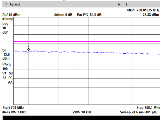
Plot 7.5.23 Spurious emissions at RF antenna connector, high channel band edge measurements
