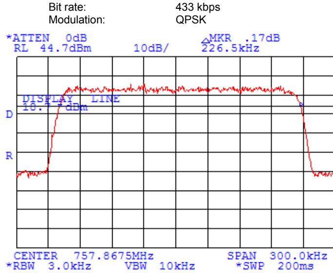
Plot 7.9.9 Occupied bandwidth test results at high frequency
