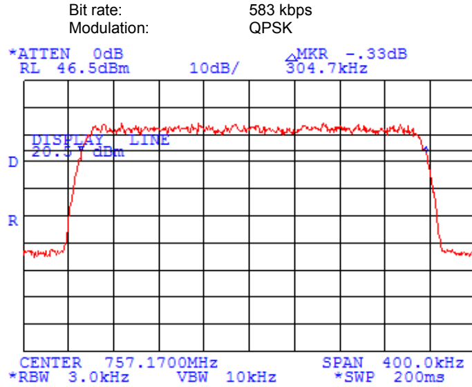
Plot 7.9.13 Occupied bandwidth test results at low frequency
