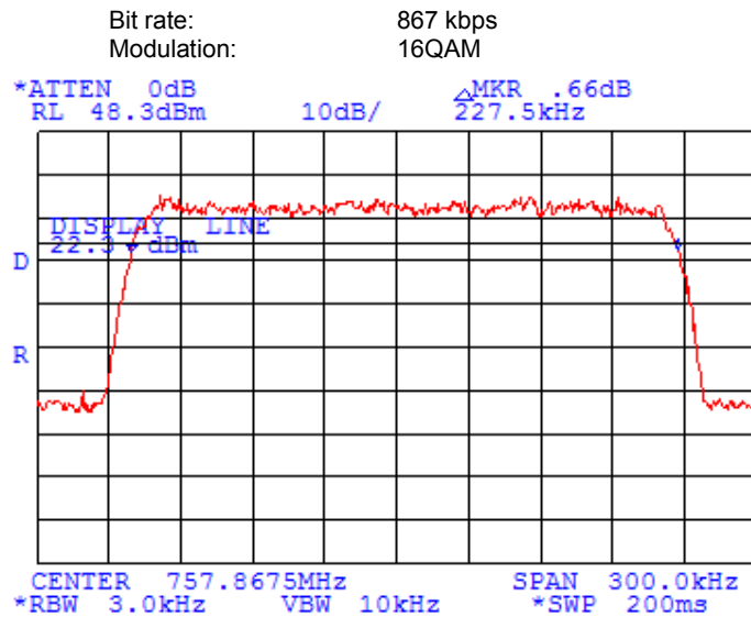
Plot 7.9.10 Occupied bandwidth test results at high frequency
