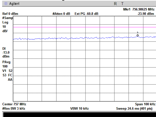
Plot 7.5.38 Spurious emissions at RF antenna connector, low channel band edge measurements
