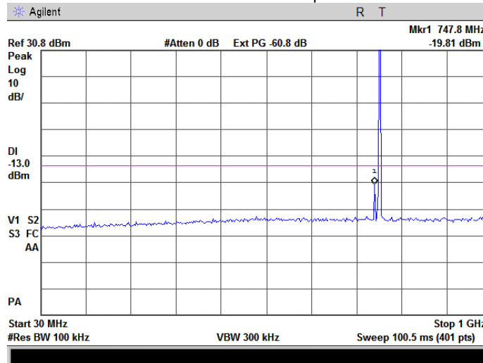
Plot 7.3.28 Spurious emission measurements at RF antenna connector, low channel
