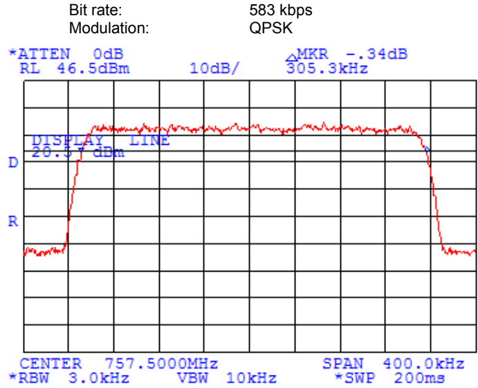
Plot 7.9.17 Occupied bandwidth test results at mid frequency
