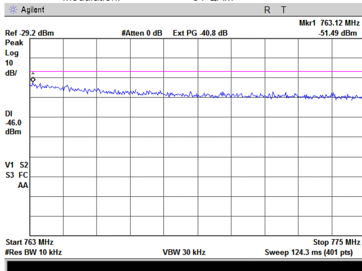
Plot 7.4.8 Spurious emission test results at low frequency
