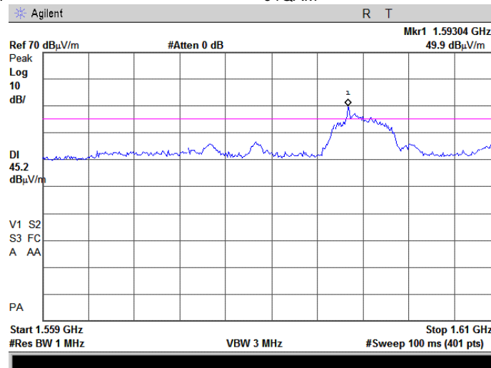
Plot 7.7.2 Signal bandwidth measurements
