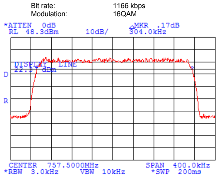
Plot 7.9.18 Occupied bandwidth test results at mid frequency
