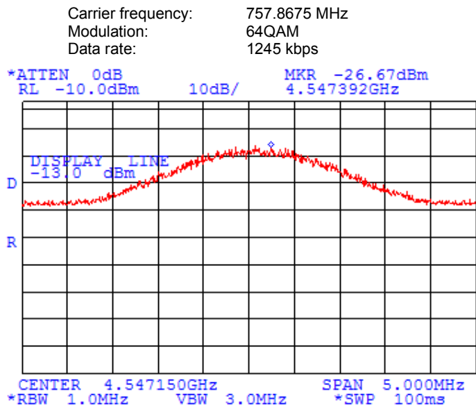
Plot 7.3.18 Spurious emission measurements at RF antenna connector, the 6 th harmonic of the high channel
