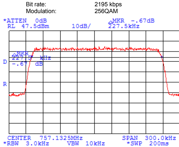
Plot 7.9.4 Occupied bandwidth test results at low frequency
