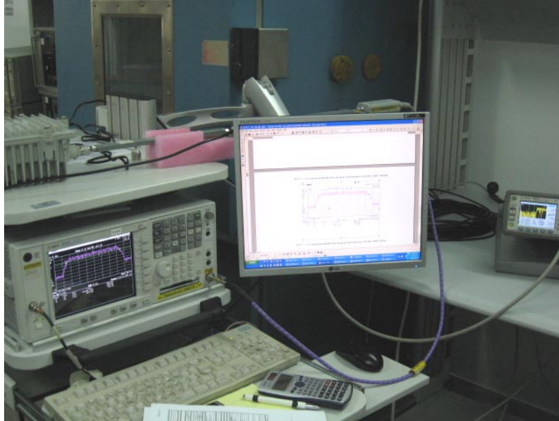
Photograph No.1 Peak output power, occupied bandwidth and spurious emissions measurements at RF antenna connector test setup
