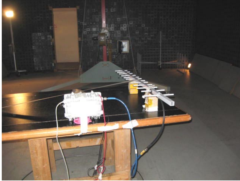
Photograph No.4 Setup for spurious emission field strength measurements in 1559-1610 MHz band
