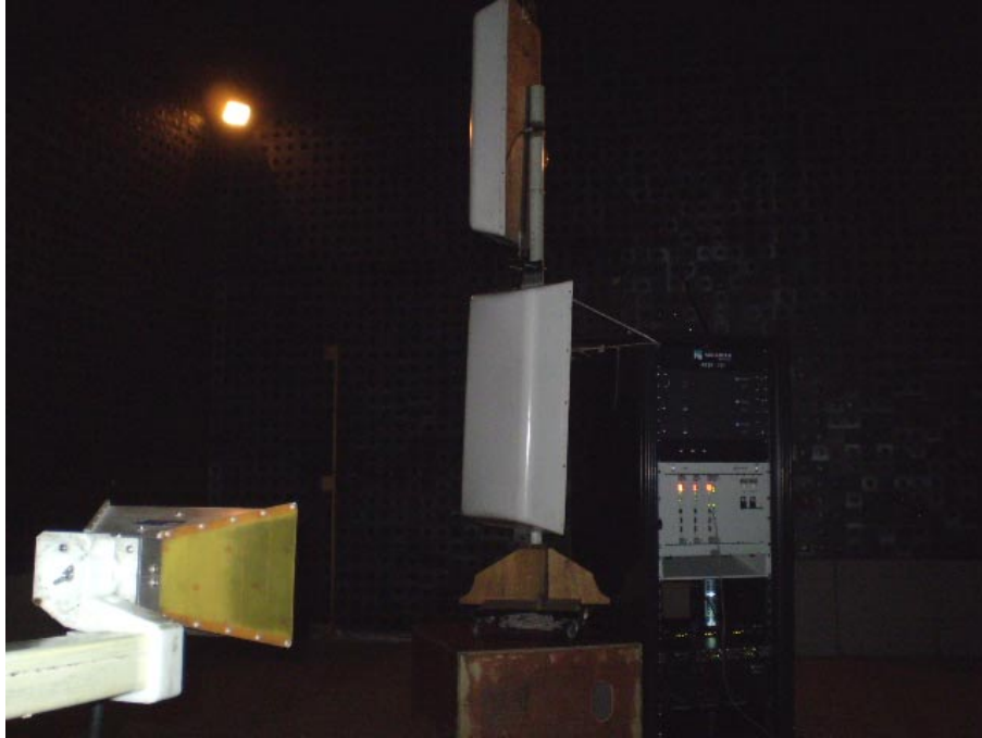
Photograph No.6 Setup for spurious emission field strength measurements in 1559 -1610 MHz band in the anechoic chamber
