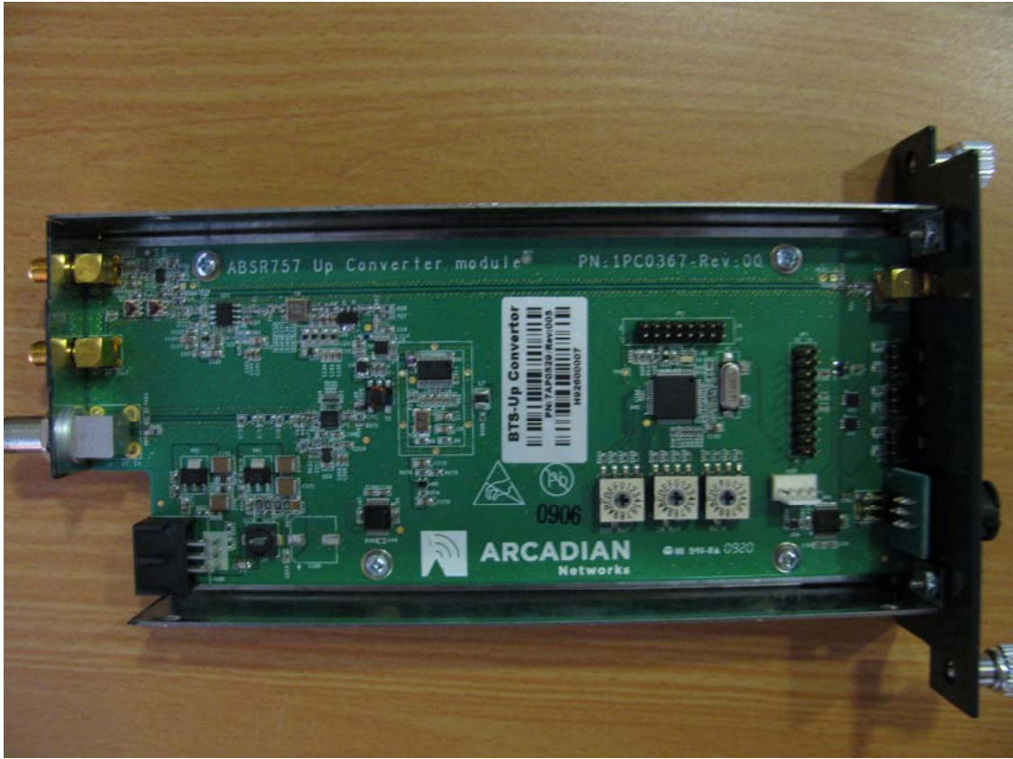
Picture 7: Upconverter module PCBA (upper cover removed)
