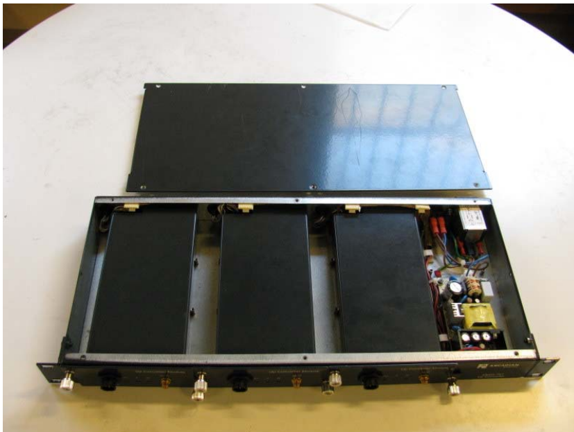
Figure 2: Upconverter front (removed cover)
