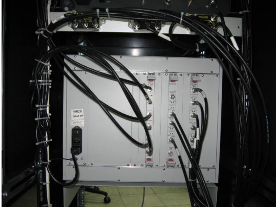
Photograph No.7 Base station ABR-757 WMTS rear side view
