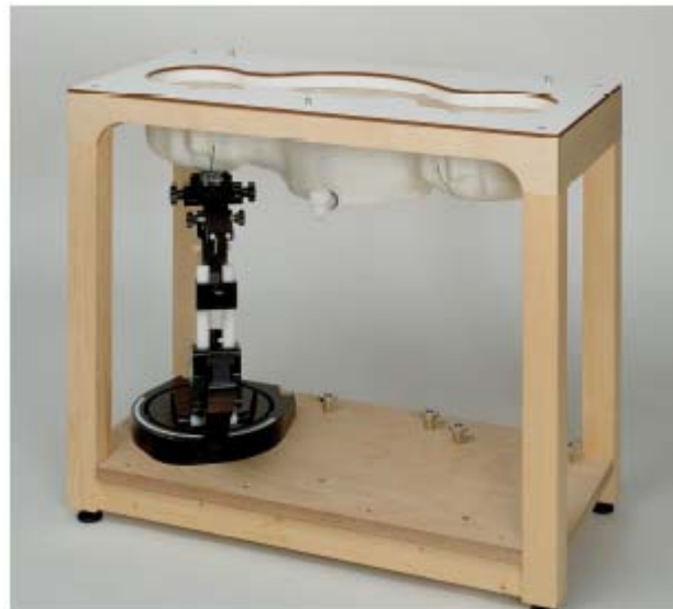
Figure 5.4 SAM Twin Phantom
