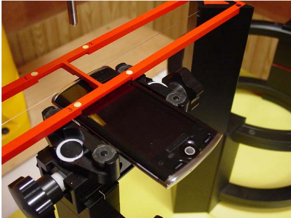
Figure 1a – HAC T-Coil Test Setup
