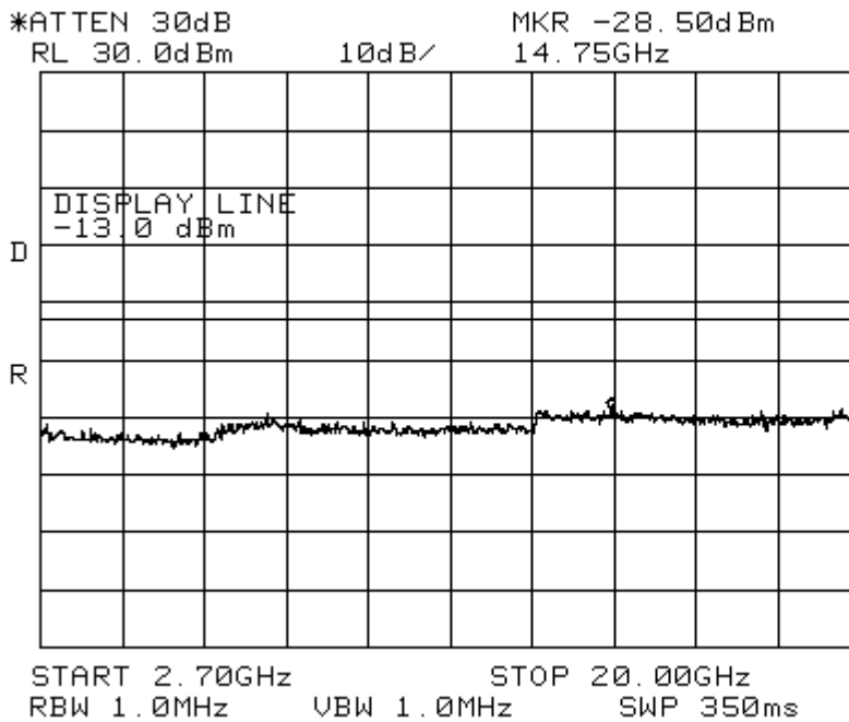
Figure 9-6b CDMA 1900 - Conducted Spurious Emission (CH 1175)
