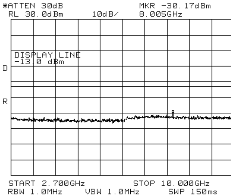
Figure 9-2b CDMA 800 – Conducted Spurious Emission (CH 383)
