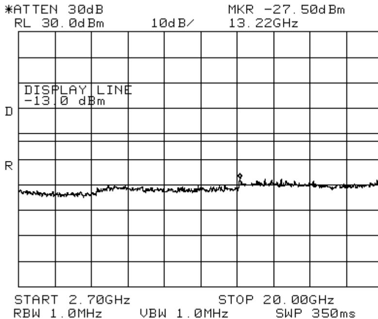
Figure 9-5b CDMA 1900 - Conducted Spurious Emission (CH 600)
