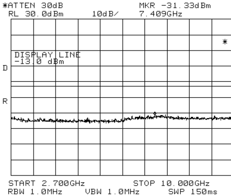
Figure 9-1b CDMA 800 – Conducted Spurious Emission (CH 1013)
