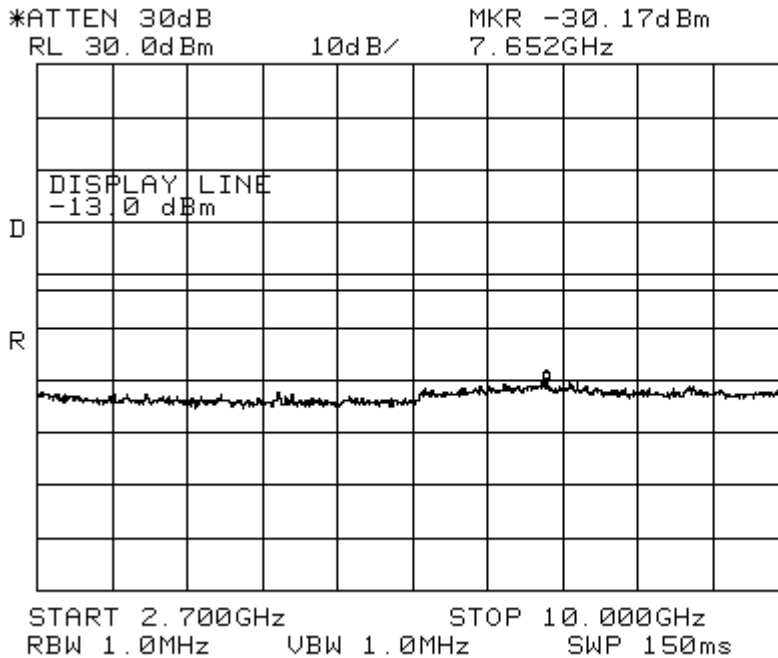
Figure 9-3b CDMA 800 – Conducted Spurious Emission (CH 777)
