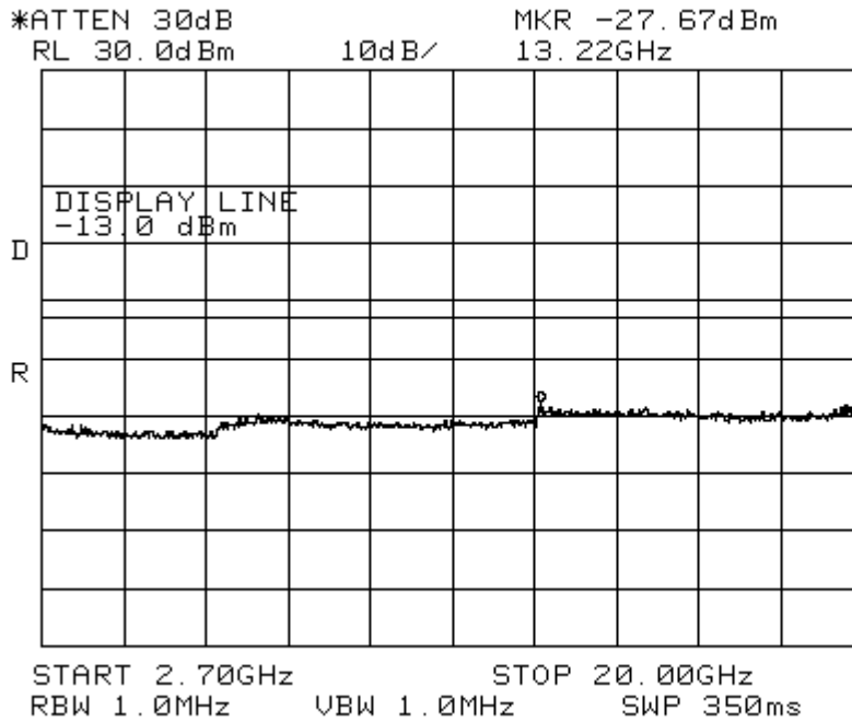
Figure 9-4b CDMA 1900 - Conducted Spurious Emission (CH 25)
