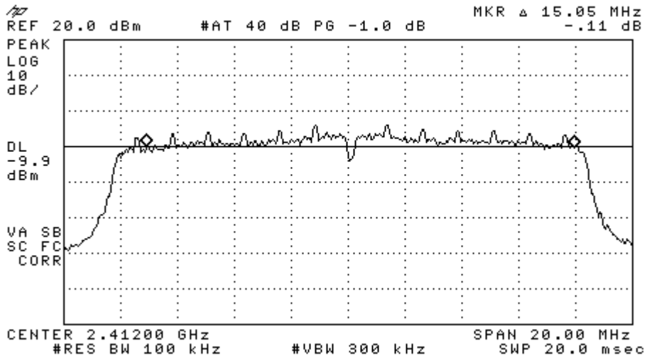
Figure 6-2a: 6 dB Bandwidth, 802.11g, Ch 1.
