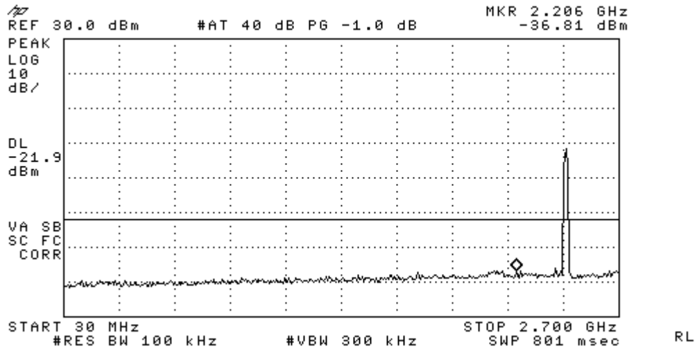
Figure 10-2b1: Conducted Spurious Emissions, 802.11g, Ch 6
