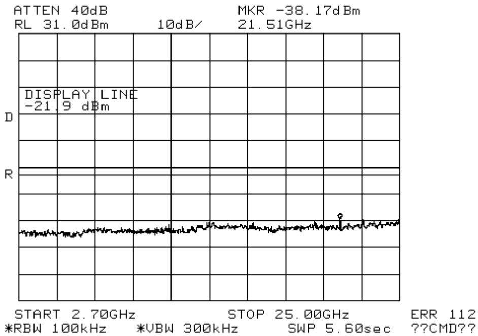
Figure 10-2b2: Conducted Spurious Emissions, 802.11g, Ch 6
