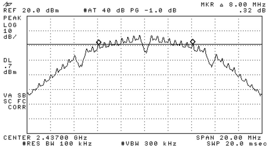
Figure 6-1b: 6 dB Bandwidth, 802.11b, Ch 6.
