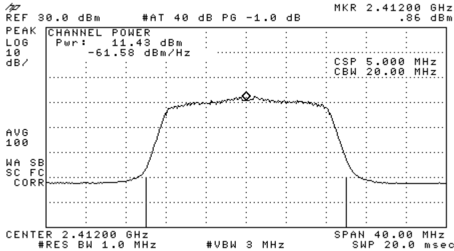
Figure 7-4: Output Power 802.11g, 6Mbps, Ch 1
