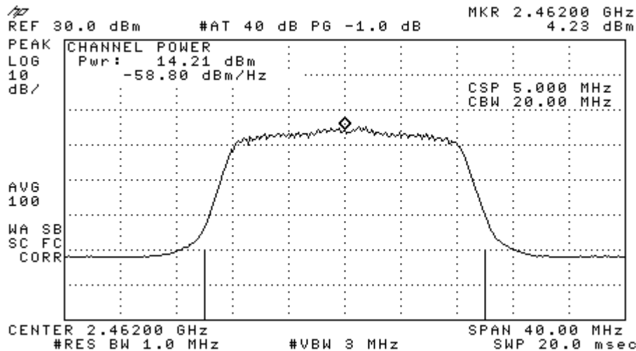
Figure 7-6: Output Power 802.11g, 6 Mbps, Ch 11
