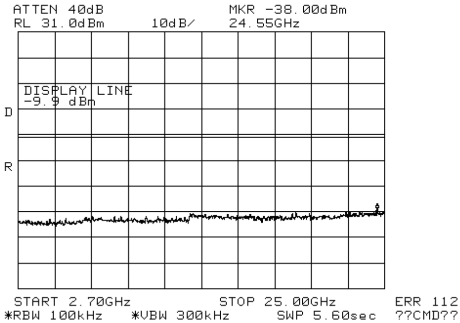
Figure 10-1a2: Conducted Spurious Emissions, 802.11b, Ch 1
