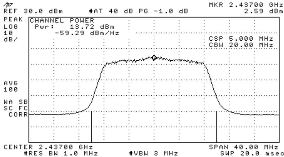
Figure 7-5: Output Power 802.11g, 6Mbps, Ch 6
