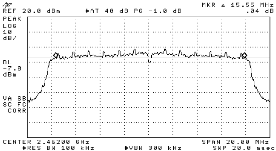
Figure 6-2c: 6 dB Bandwidth, 802.11g, Ch 11.
