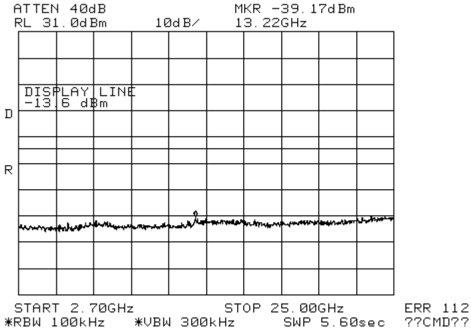
Figure 10-1b2: Conducted Spurious Emissions, 802.11b, Ch 6
