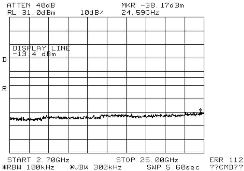
Figure 10-1c2: Conducted Spurious Emissions, 802.11b, Ch 11
