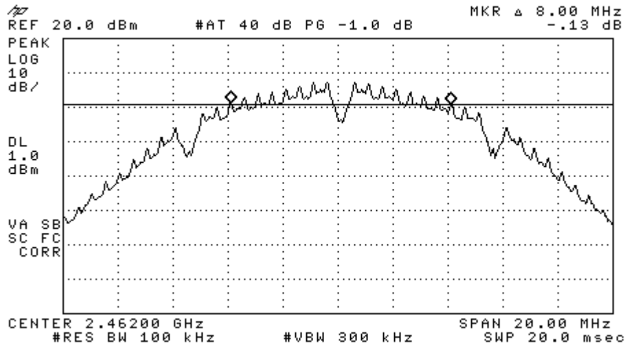
Figure 6-1c: 6 dB Bandwidth, 802.11b, Ch 11.
