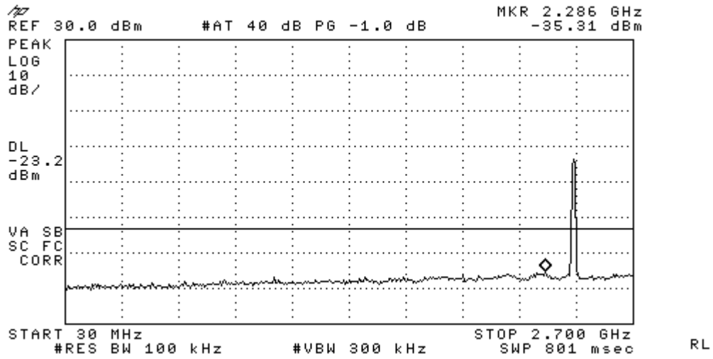
Figure 10-2a: Conducted Spurious Emissions, 802.11g, Ch 1
