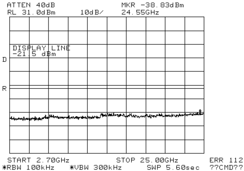
Figure 10-2c2: Conducted Spurious Emissions, 802.11g, Ch 11
