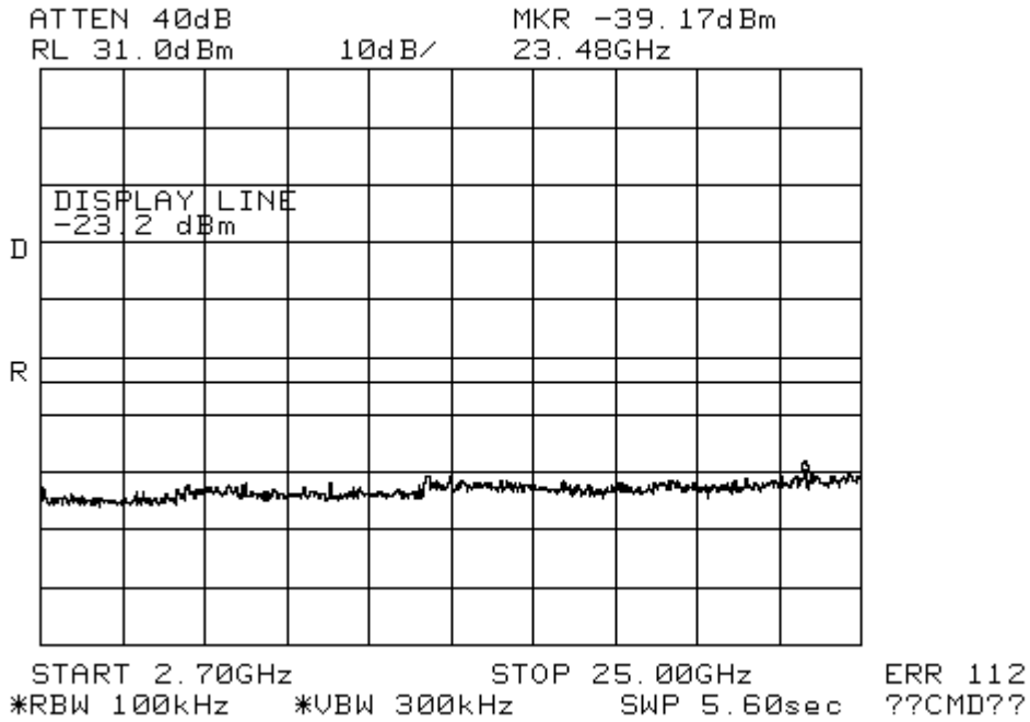
Figure 10-2a: Conducted Spurious Emissions, 802.11g, Ch 1
