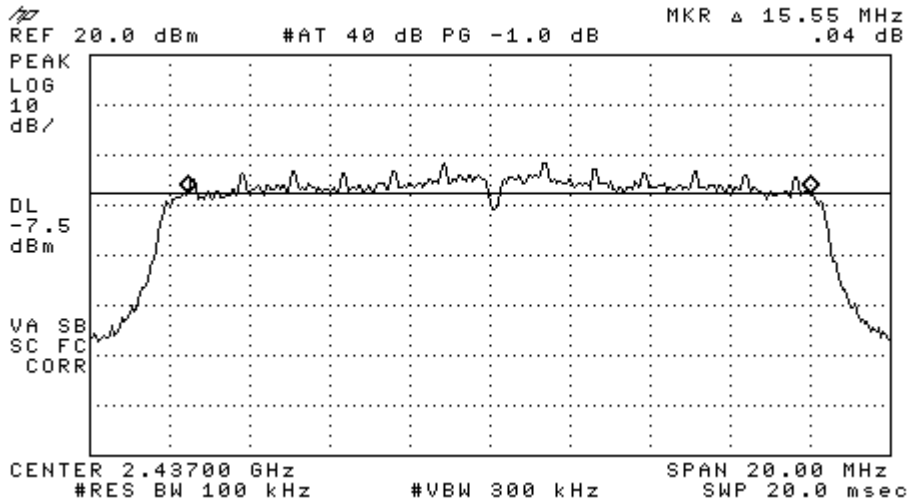
Figure 6-2b: 6 dB Bandwidth, 802.11g, Ch 6.
