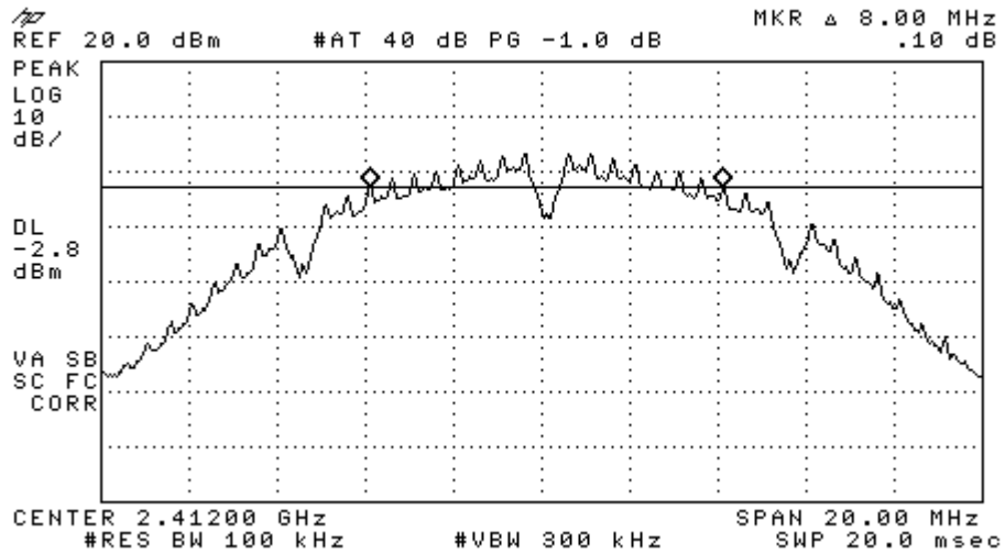
Figure 6-1a: 6 dB Bandwidth, 802.11b, Ch 1.
