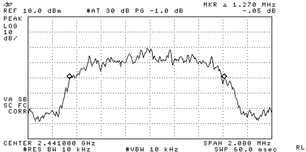
Figure 6-2b: 20dB Bandwidth EDR DQPSK, Channel 39.
