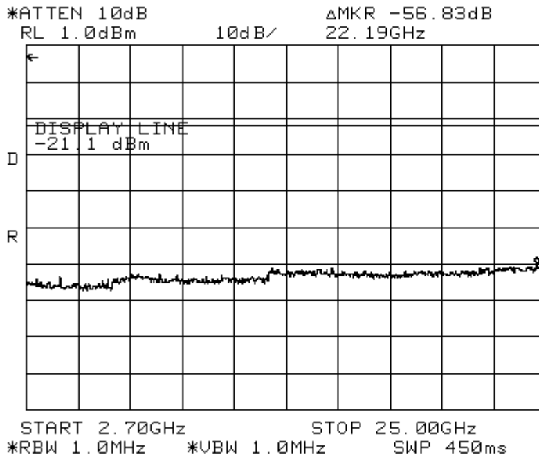
Figure 11-1b: Conducted Spurious Emissions (CH 0).
