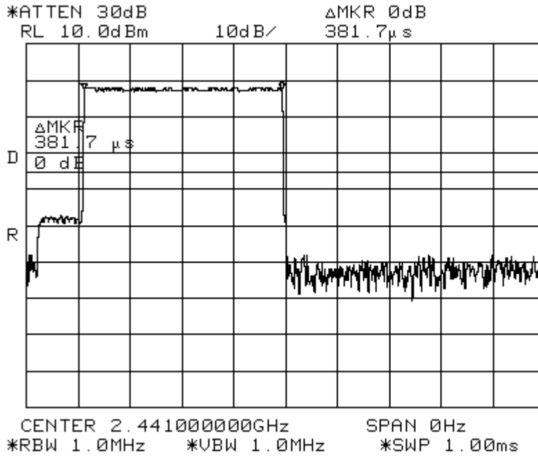
Figure 9: Duration of one transmission (Channel 39).
