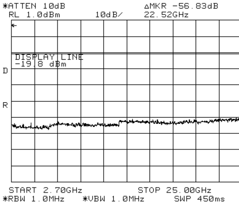
Figure 11-3b: Conducted Spurious Emissions (CH 78).
