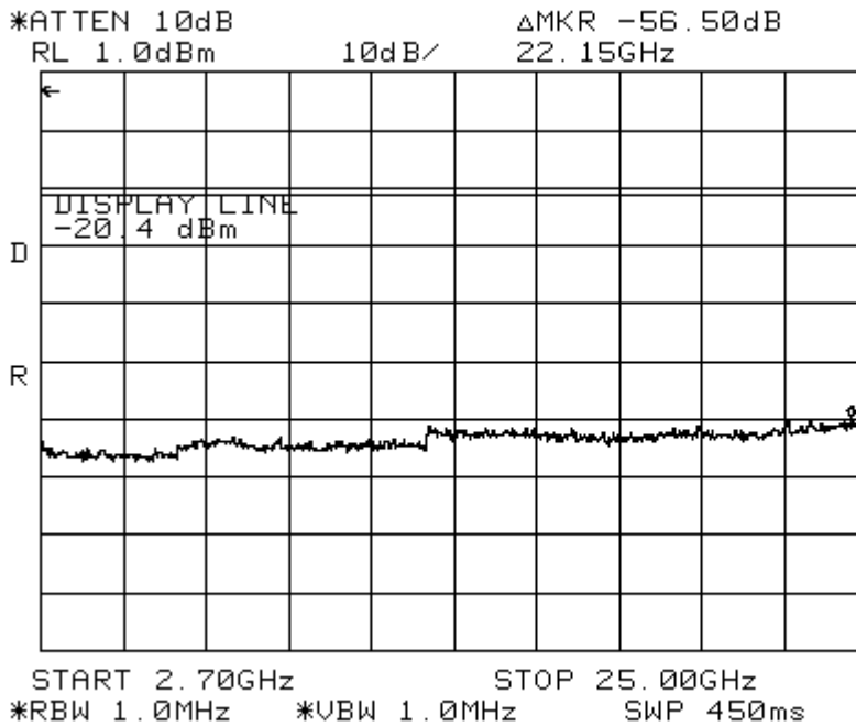
Figure 11-2b: Conducted Spurious Emissions (CH 39).
