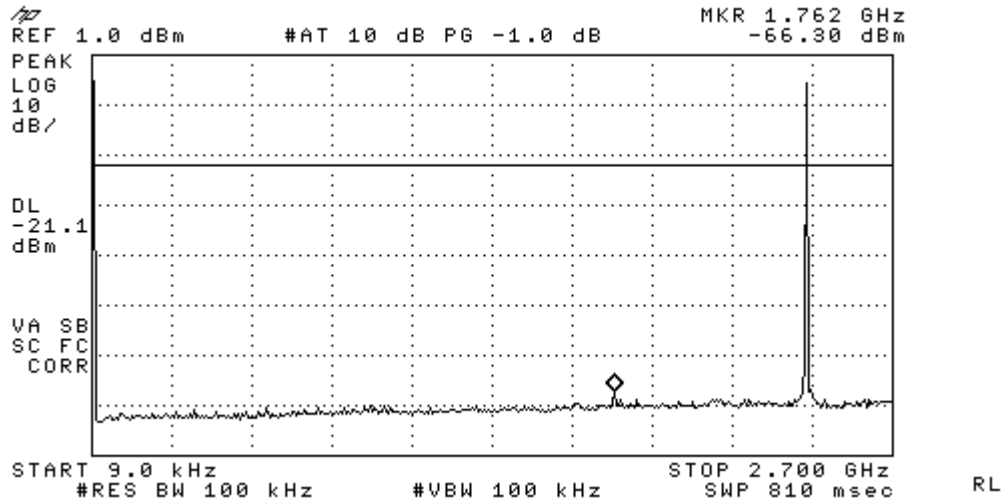
Figure 11-1a: Conducted Spurious Emissions (CH 0).
