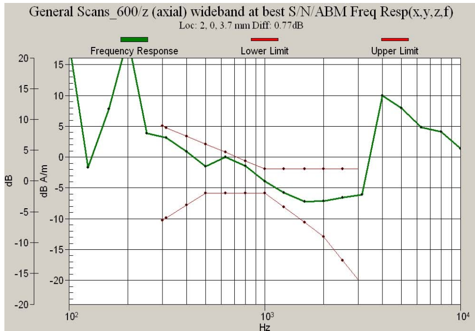
Figure 9.2b CDMA 1900 Frequency Response
