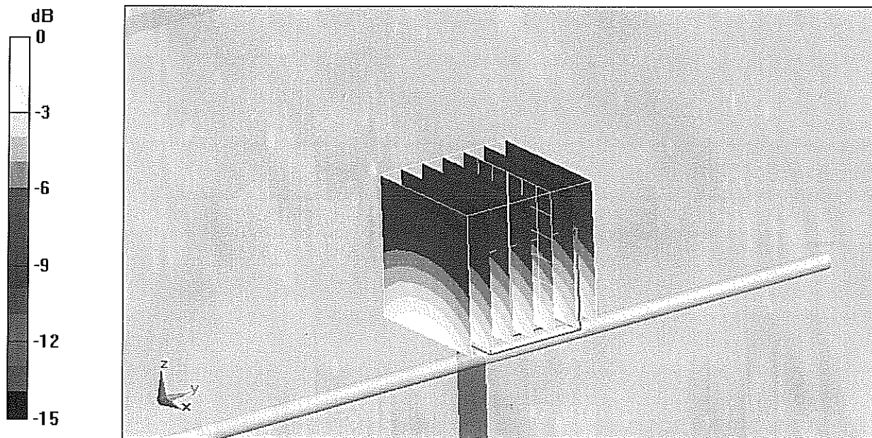
0 dB = 2.73mW/g
