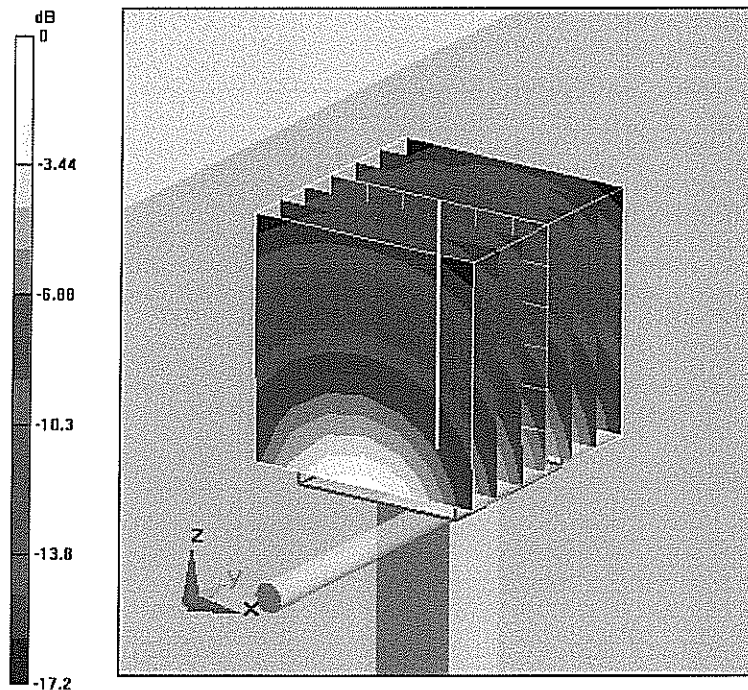
0 dB = 12.5mW/g
