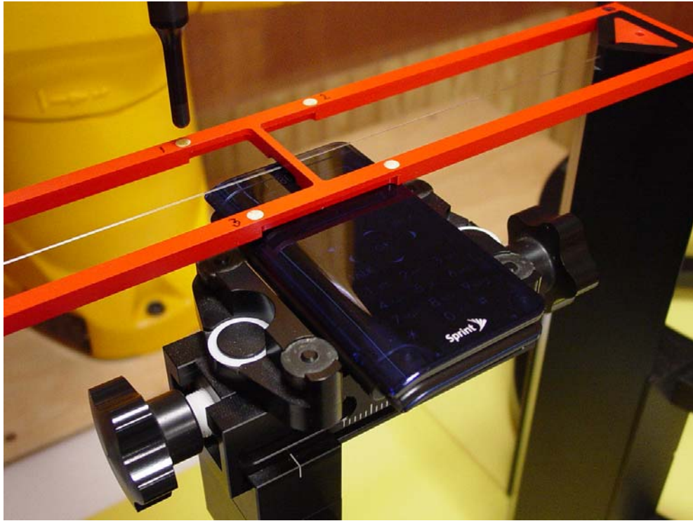
Figure 1a – HAC RF Test Setup
