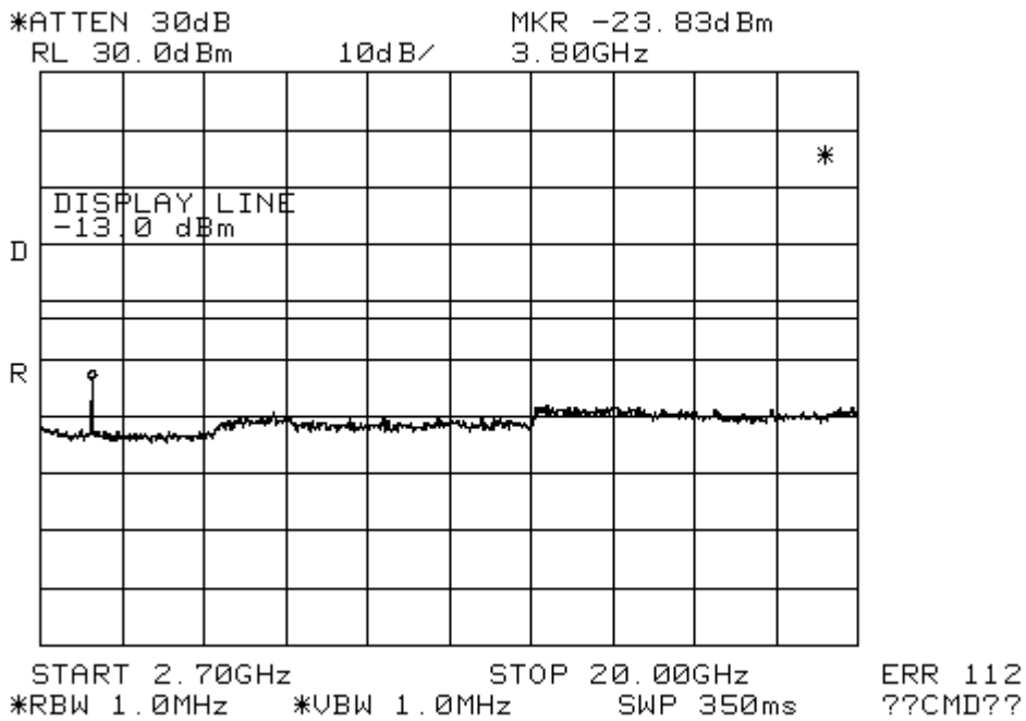
Figure 9-6b CDMA 1900 - Conducted Spurious Emission (CH 1175)
