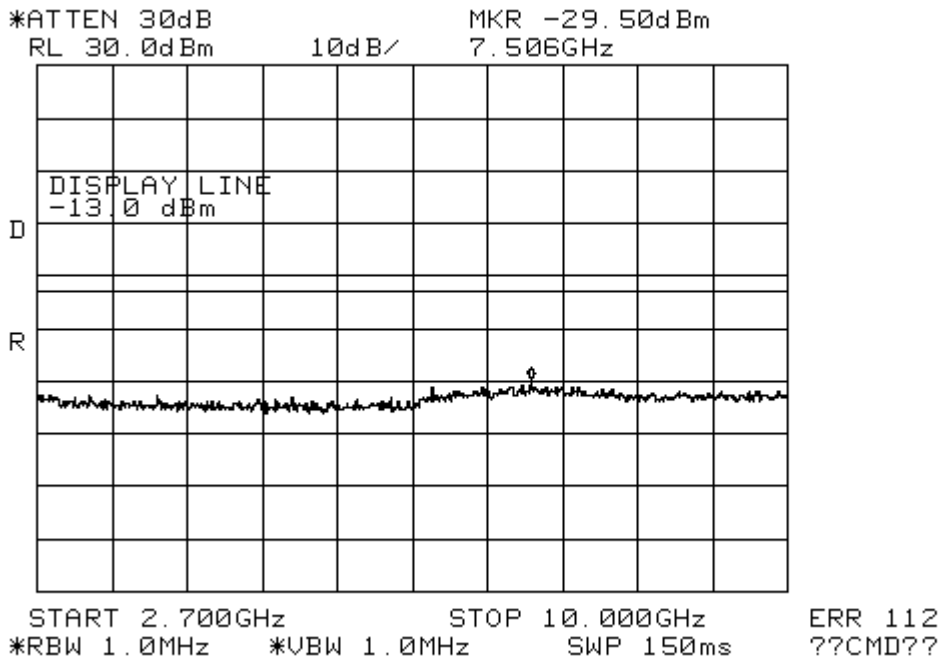
Figure 9-2b CDMA 800 – Conducted Spurious Emission (CH 383)
