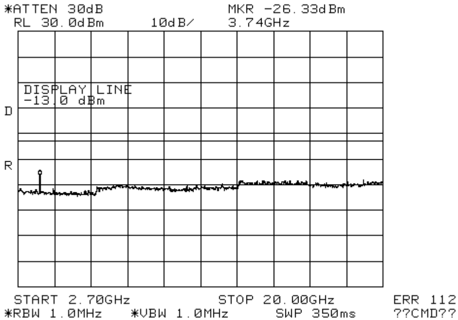
Figure 9-5b CDMA 1900 - Conducted Spurious Emission (CH 600)
