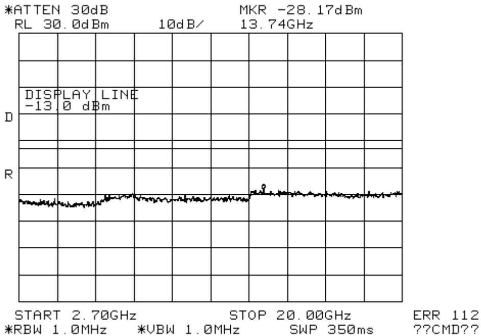
Figure 9-4b CDMA 1900 - Conducted Spurious Emission (CH 25)
