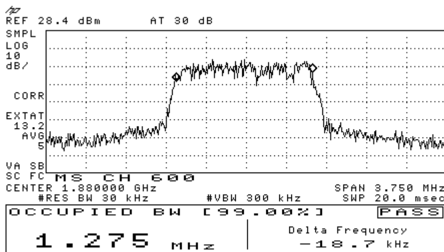
Figure 8-4 CDMA 1900 @ CH 600
