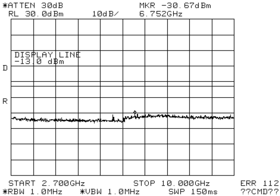
Figure 9-3b CDMA 800 – Conducted Spurious Emission (CH 777)
