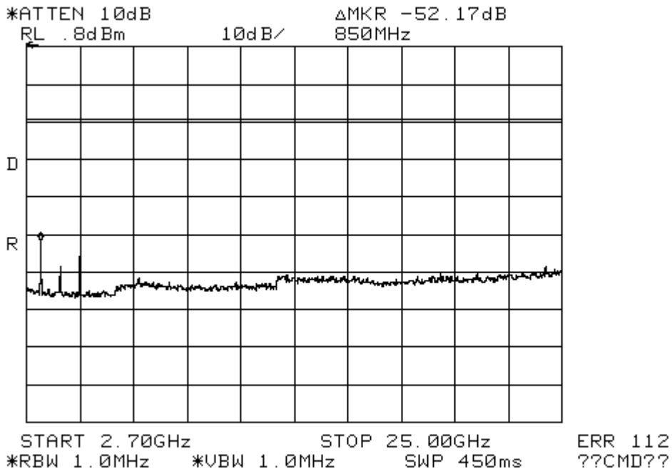
Figure 11-3b: Conducted Spurious Emissions (CH 78).
