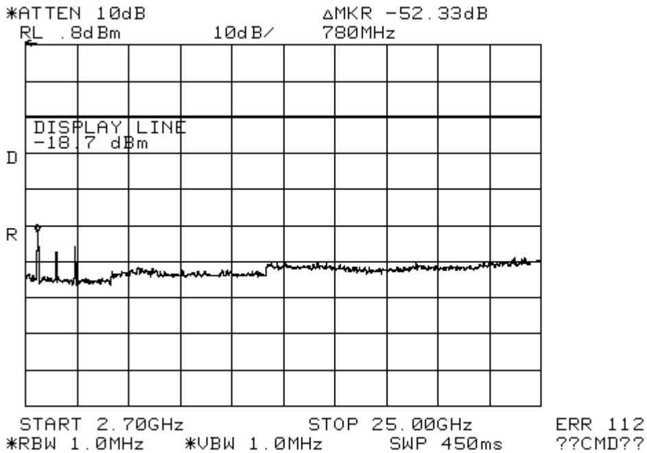
Figure 11-2b: Conducted Spurious Emissions (CH 39).
