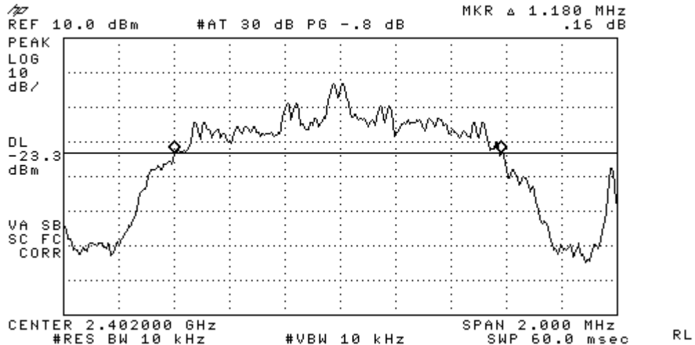
Figure 6-1b: 20dB Bandwidth EDR DQPSK, Channel 0.
