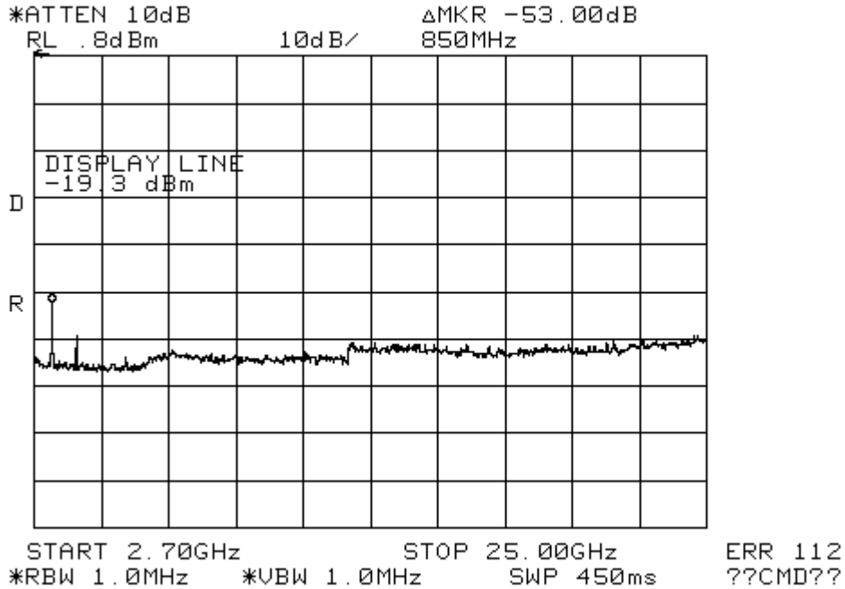
Figure 11-1b: Conducted Spurious Emissions (CH 0).
