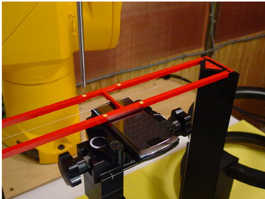
Figure 1b – HAC T-Coil Test Setup
