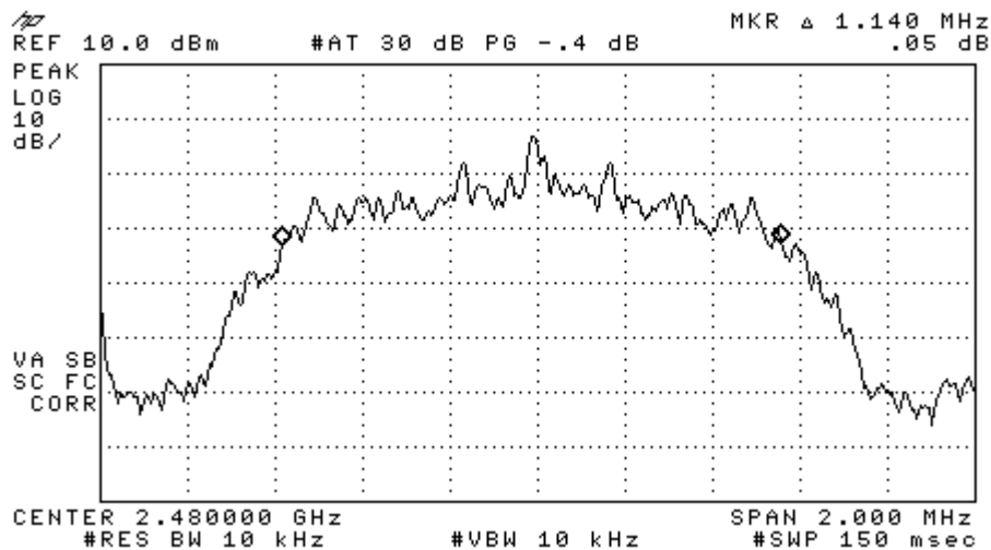
Figure 6-3c: 20dB Bandwidth EDR D8PSK, Channel 78.
