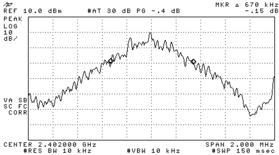
Figure 6-1a: 20dB Bandwidth Basic rate, Channel 0.
