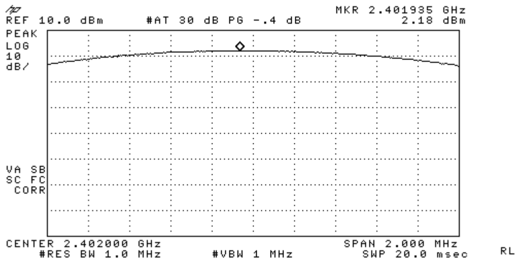
Figure 5-1b: Peak Output Power, EDR DQPSK Channel 0.
