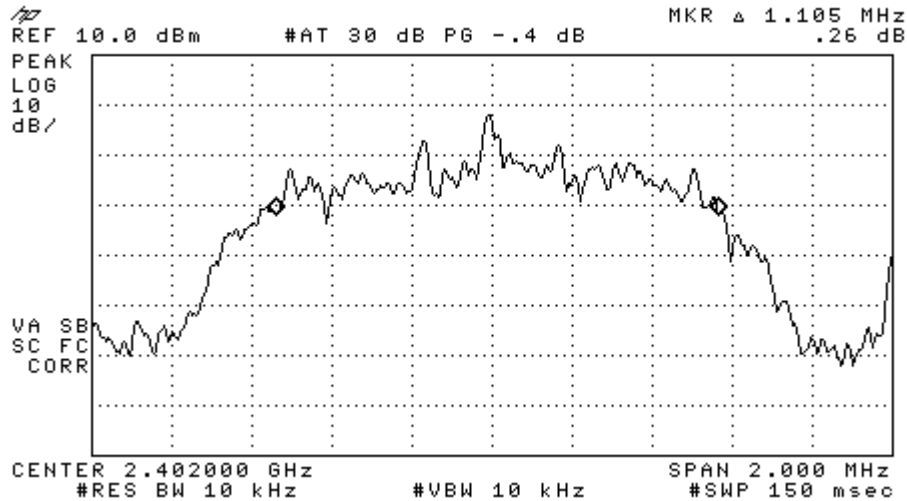
Figure 6-1b: 20dB Bandwidth EDR DQPSK, Channel 0.
