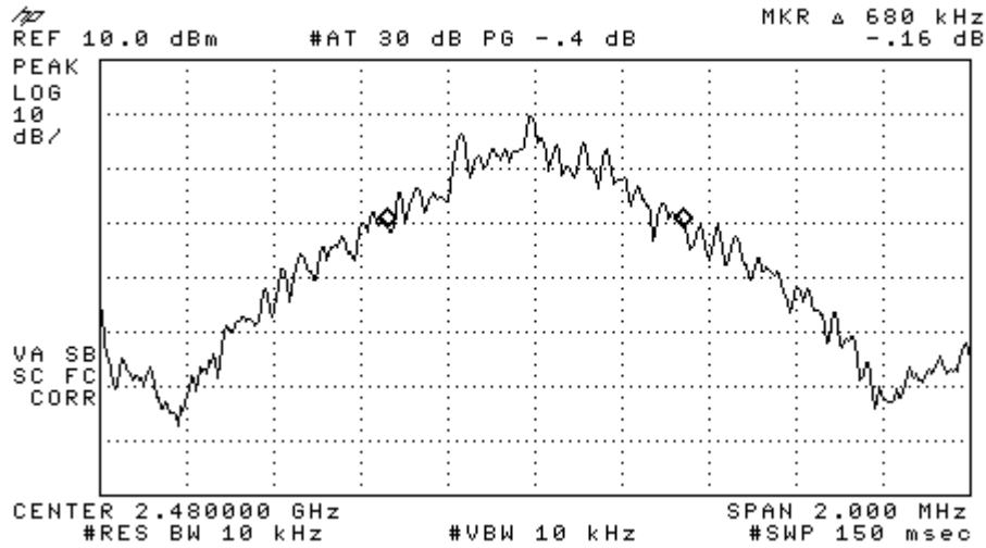
Figure 6-3a: 20dB Bandwidth Basic rate, Channel 78.
