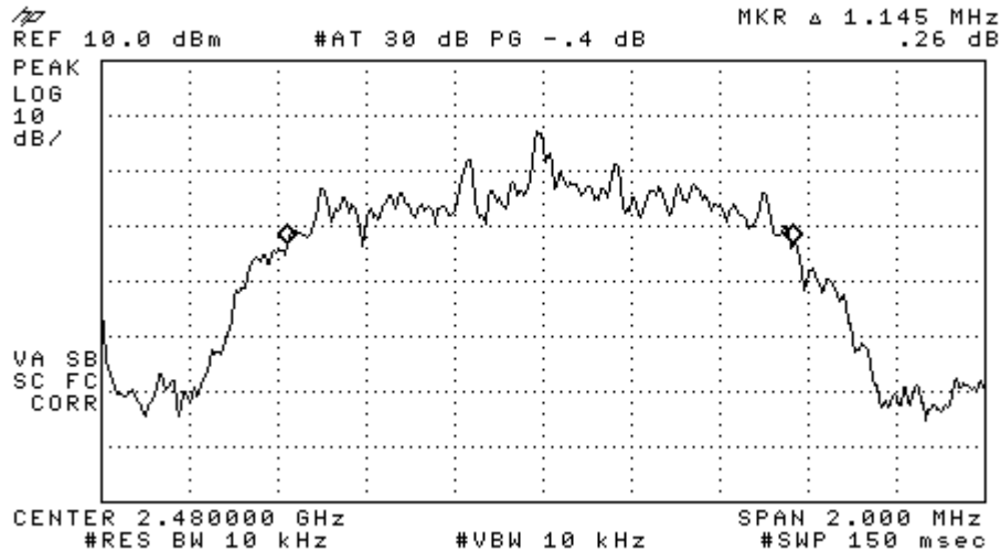
Figure 6-3b: 20dB Bandwidth EDR DQPSK, Channel 78.
