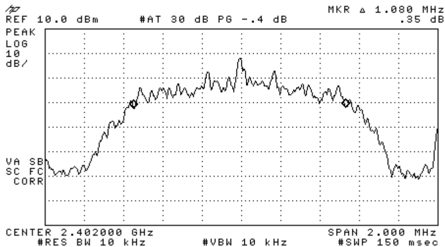
Figure 6-1c: 20dB Bandwidth EDR D8PSK, Channel 0.
