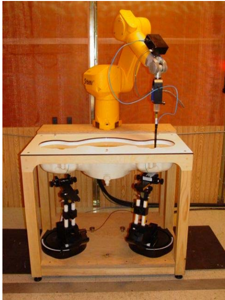
Figure 5.1 DASY 4 System
