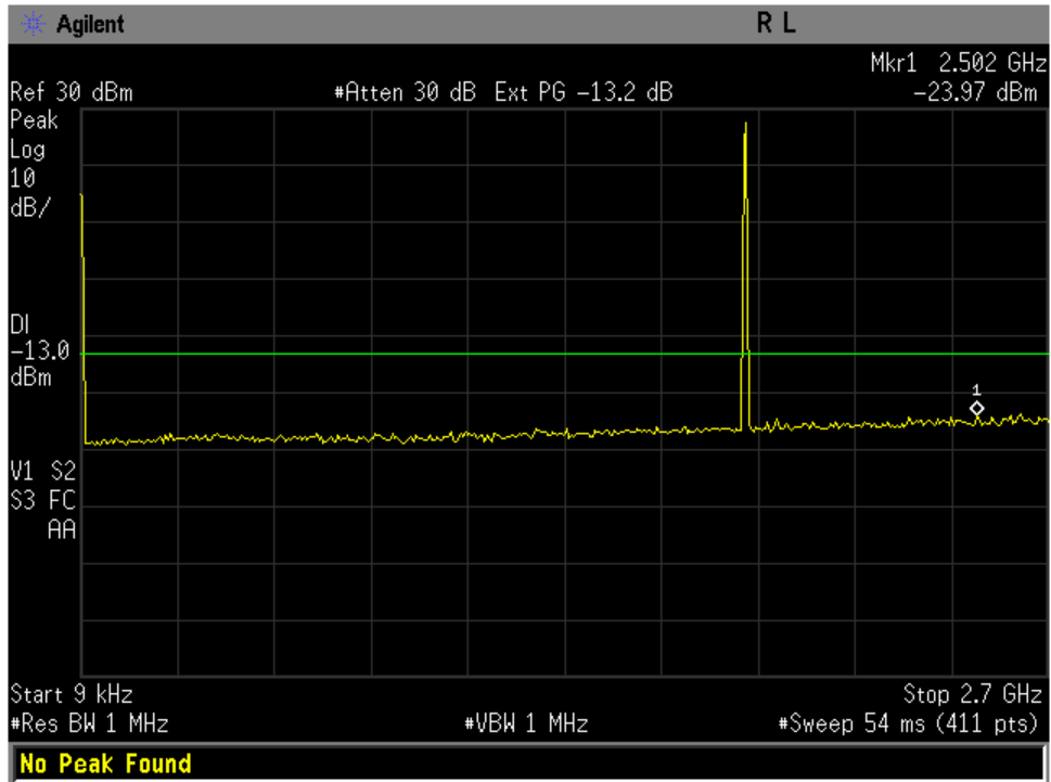
Figure 9-4a CDMA 1900 - Conducted Spurious Emission (CH 25)
