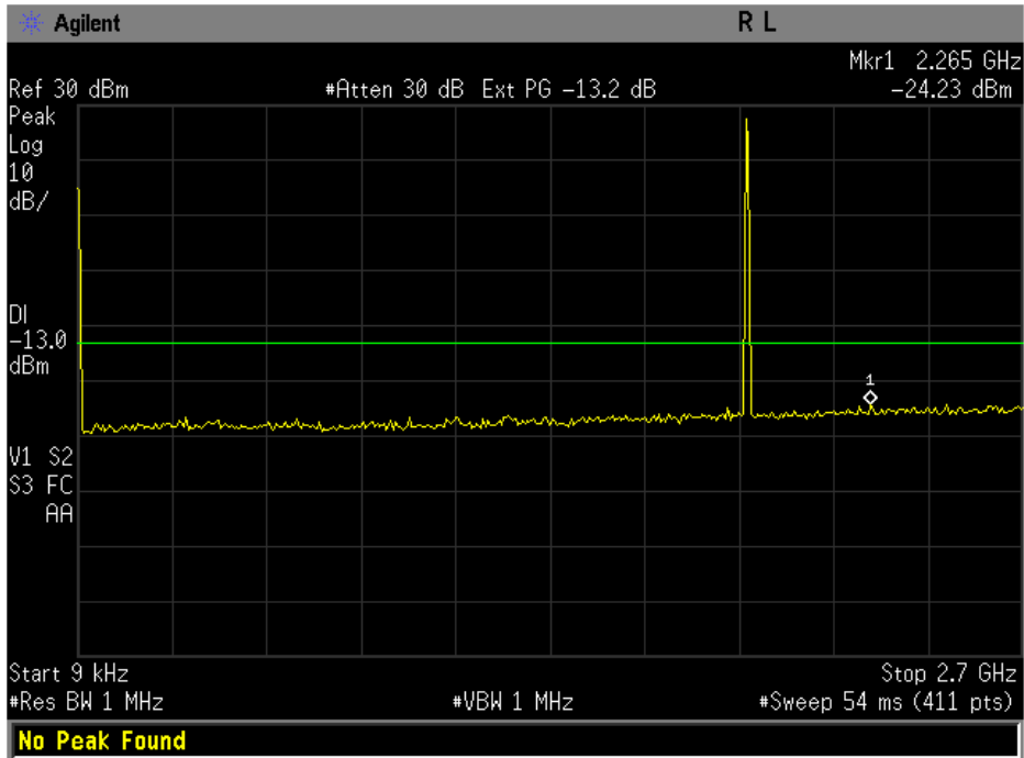
Figure 9-6a CDMA 1900 - Conducted Spurious Emission (CH 1175)
