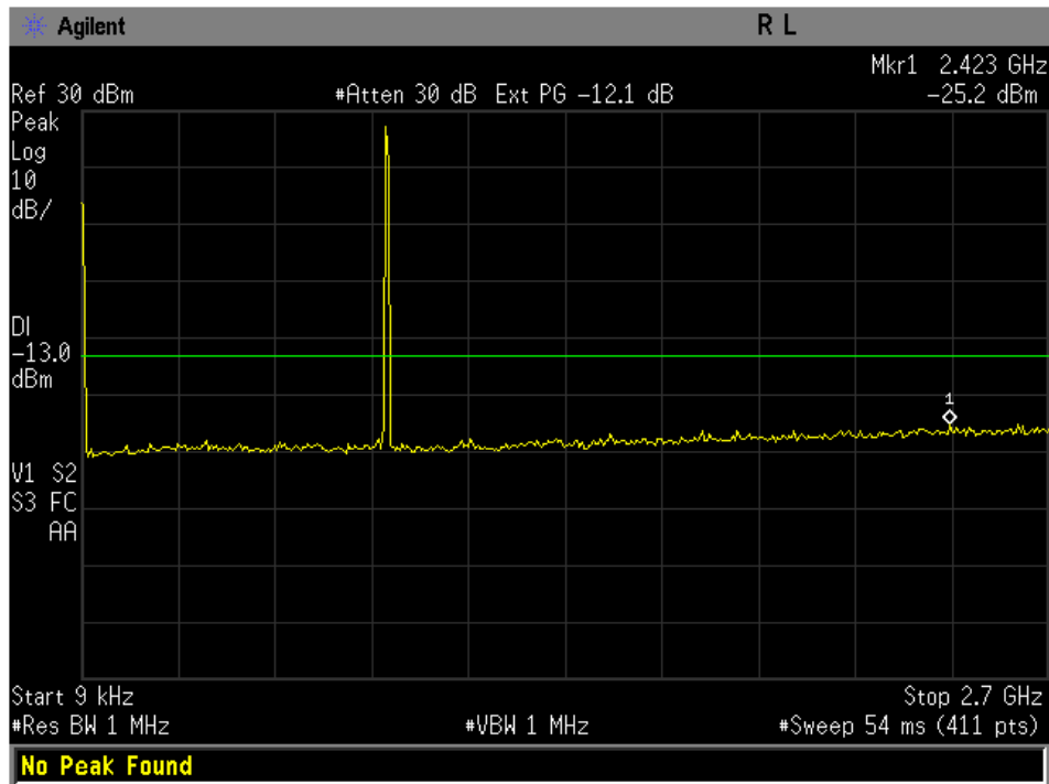
Figure 9-3a CDMA 800 – Conducted Spurious Emission (CH 777)
