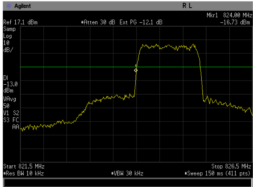
Figure 8-2 CDMA 800 Lower Band Edge @ CH 1013
