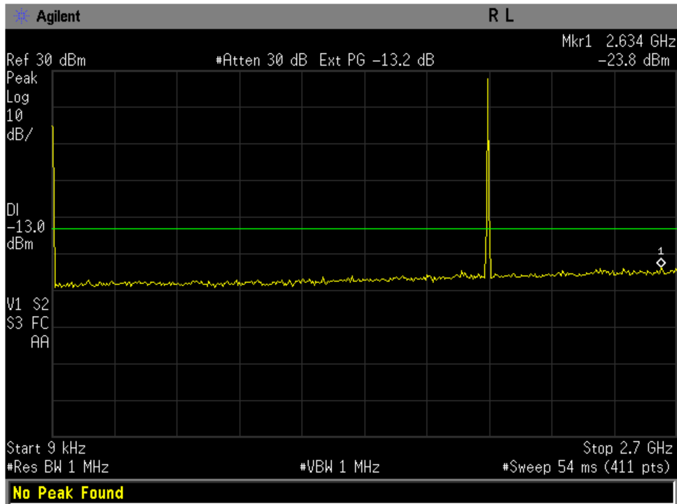
Figure 9-5a CDMA 1900 - Conducted Spurious Emission (CH 600)
