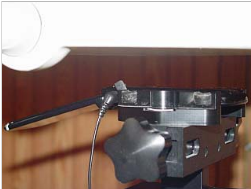
Figure 9E.4 Body SAR setup (Open, Face Down, 22mm Air Separation)
