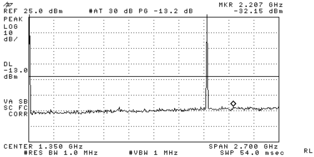
Figure 9-9a CDMA 1900 - Conducted Spurious Emission (CH 1175)
