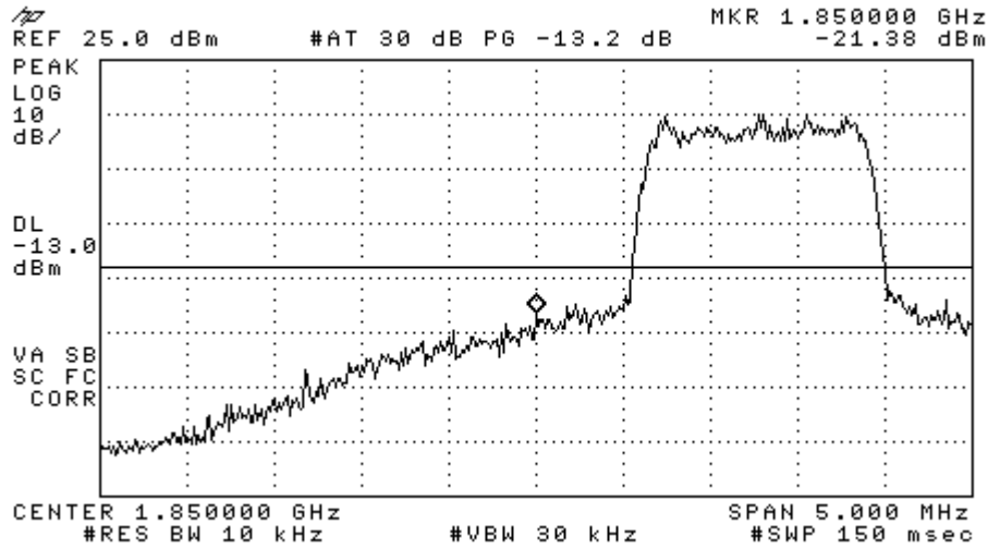
Figure 8-8 CDMA 1900 Lower Band Edge @ CH 25
