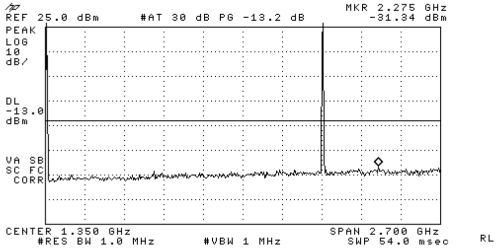
Figure 9-8a CDMA 1900 - Conducted Spurious Emission (CH 600)
