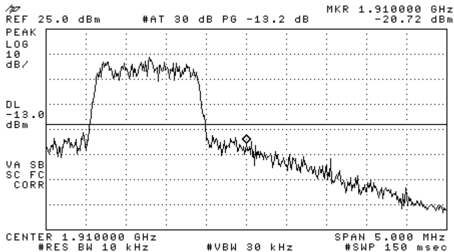
Figure 8-9 CDMA 1900 Upper Band Edge @ CH 1175
