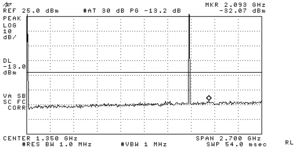
Figure 9-7a CDMA 1900 - Conducted Spurious Emission (CH 25)
