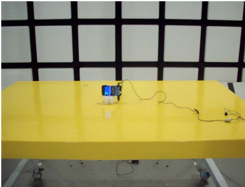
RADIATED EMISSIONS (Y-POSITION WITH CHARGER)
