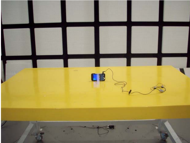
RADIATED EMISSIONS (Y-POSITION)
