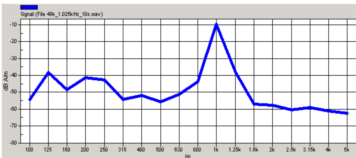
Figure 7.2a 1.025 KHz Voice signal spectrum
