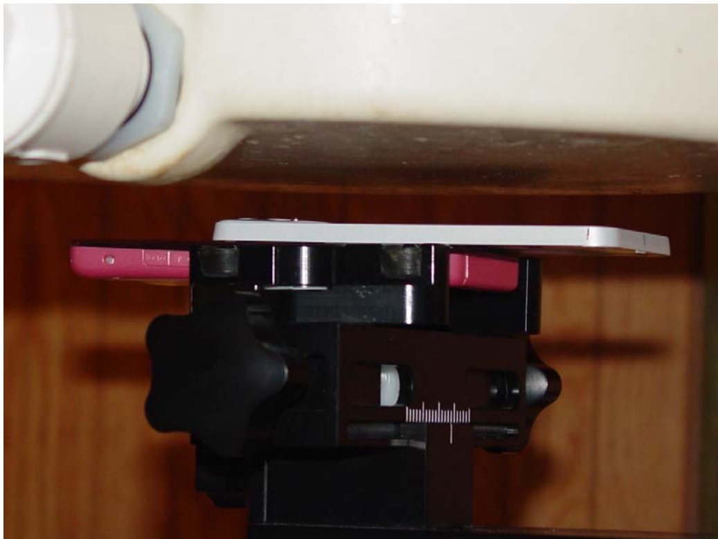
Figure 9E.8 Body SAR setup (Open, Face Up, 15mm Air Separation)
