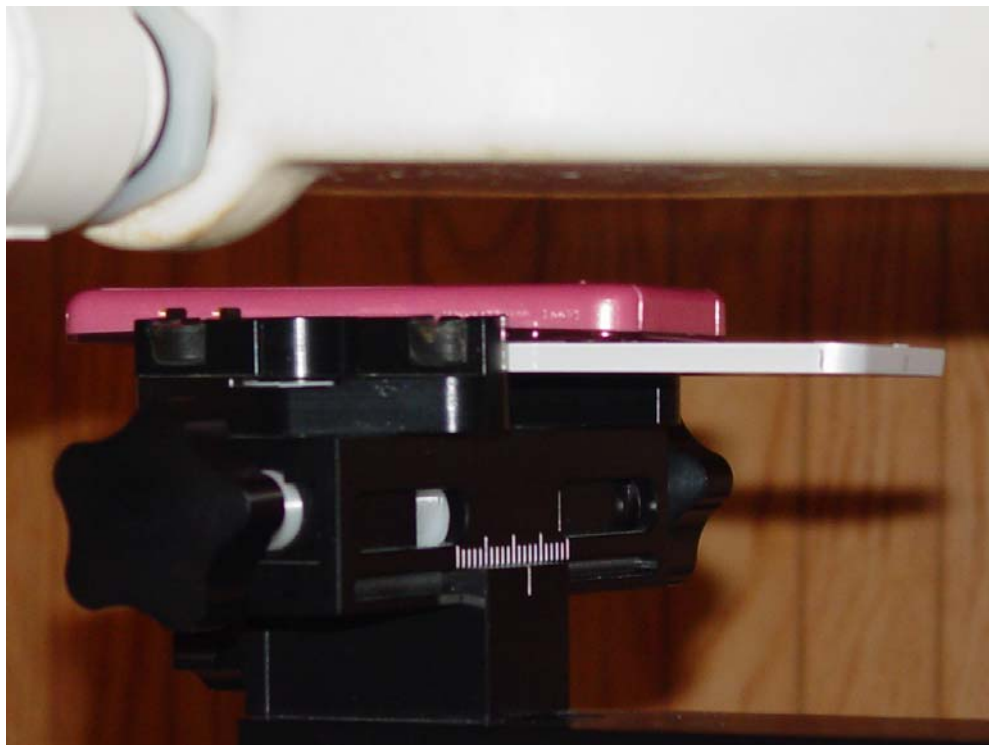
Figure 9E.6 Body SAR setup (Open, Face Down, 15mm Air Separation)
