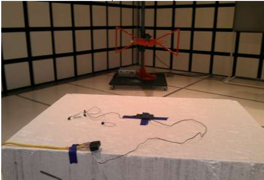
RADIATED BACK PHOTO (BELOW 1 GHz)
