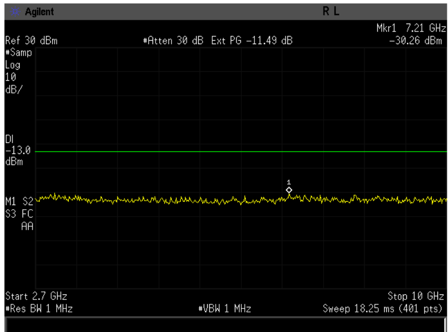
Figure 9-1b CDMA 800 BC-10 – Conducted Spurious Emission (CH 476)
