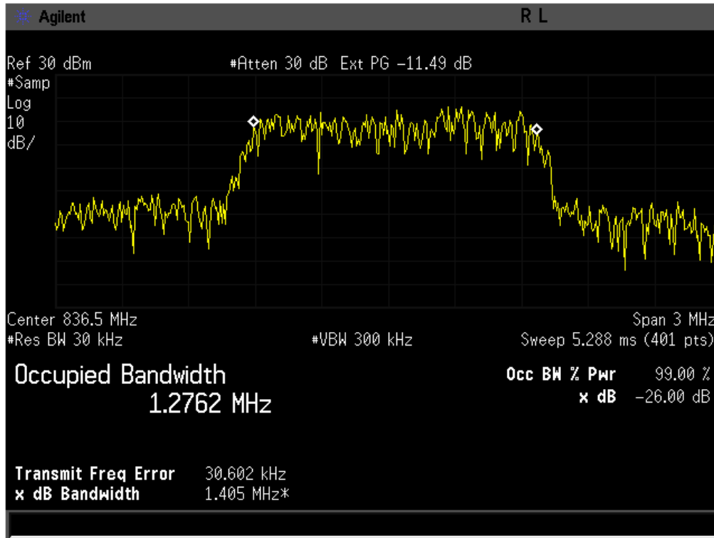
Figure 8-1 CDMA 800 @ CH 384
