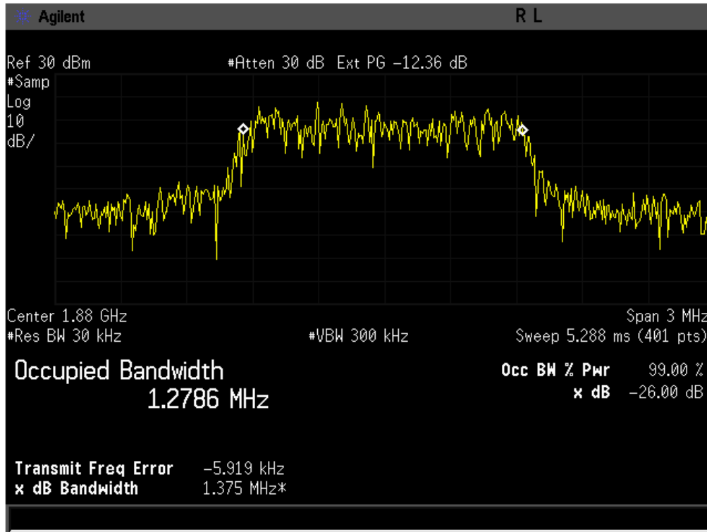
Figure 8-4 CDMA 1900 @ CH 600
