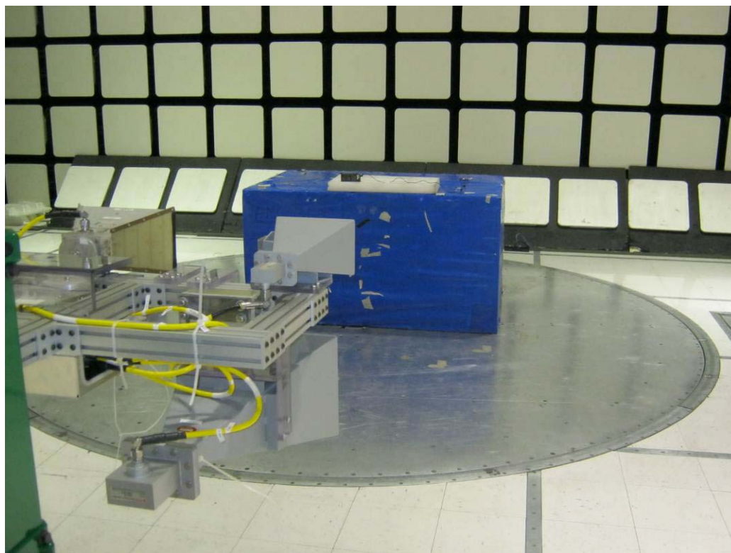
Figure 2 Test setup for Radiated Emissions
