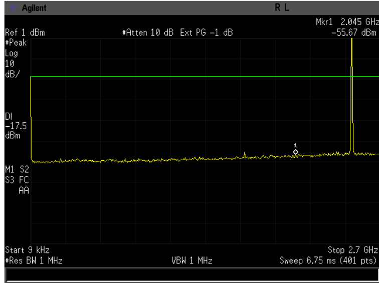
Figure 11-3a: Conducted Spurious Emissions (CH 78).
