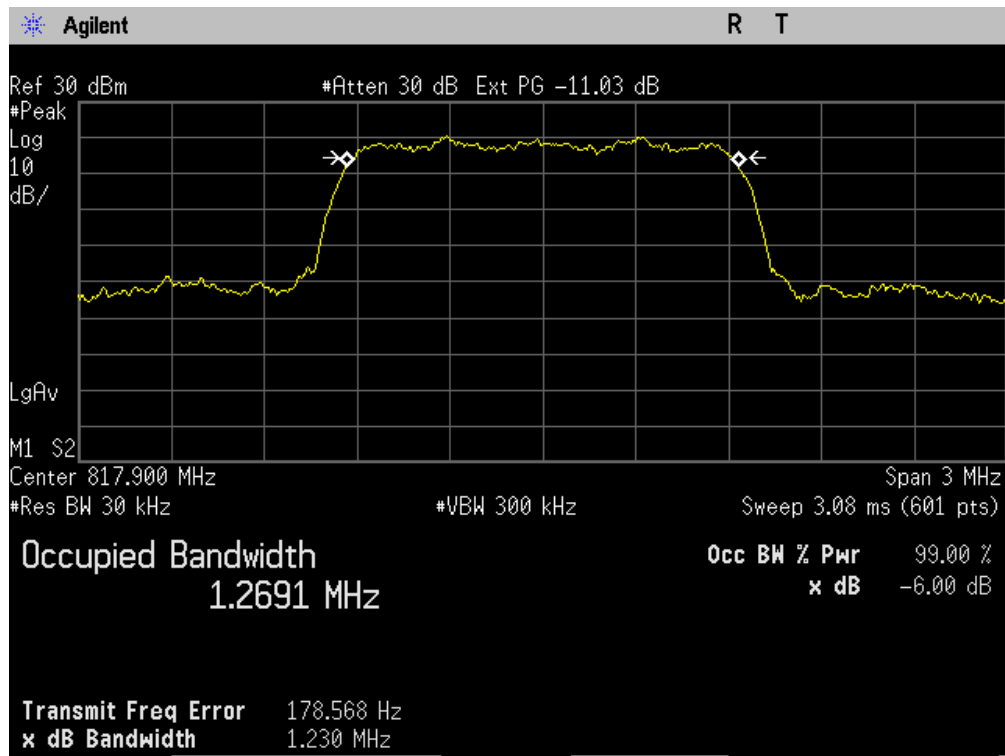
Figure 7-1 CDMA 800 BC-10 @ CH 476
