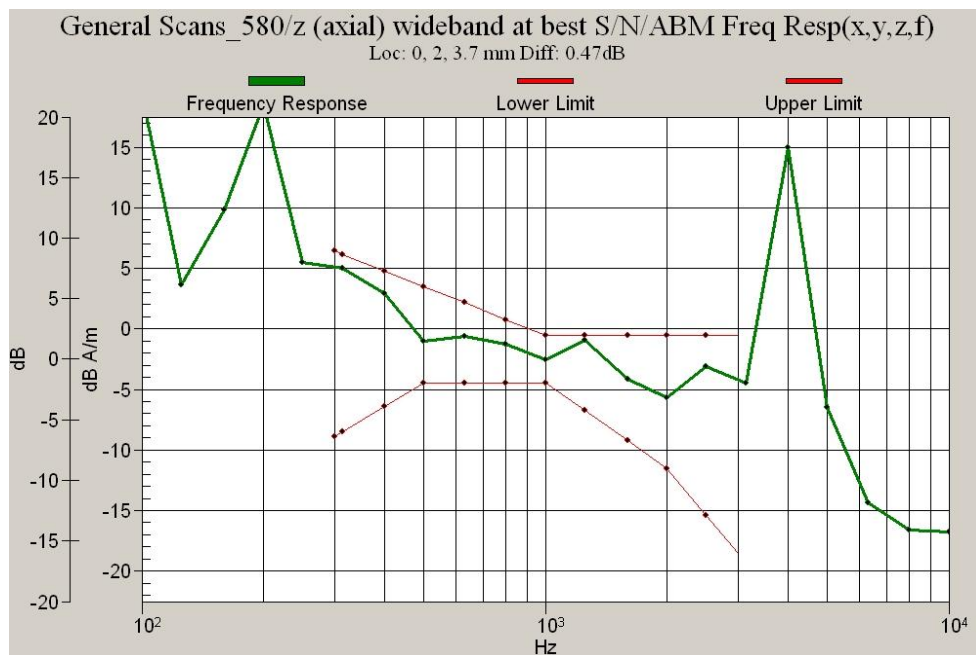
Figure 9.2b CDMA 800 BC-10, Frequency Response
