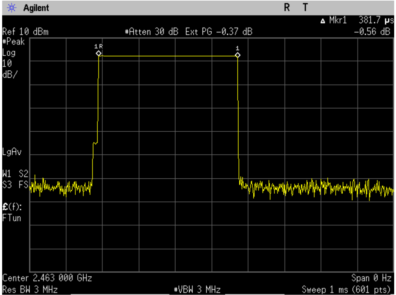
Figure 9: Duration of one transmission (Channel 39).
