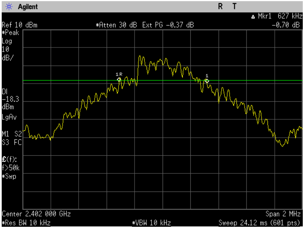
Figure 6-1a: 20dB Bandwidth Basic rate, Channel 0.
