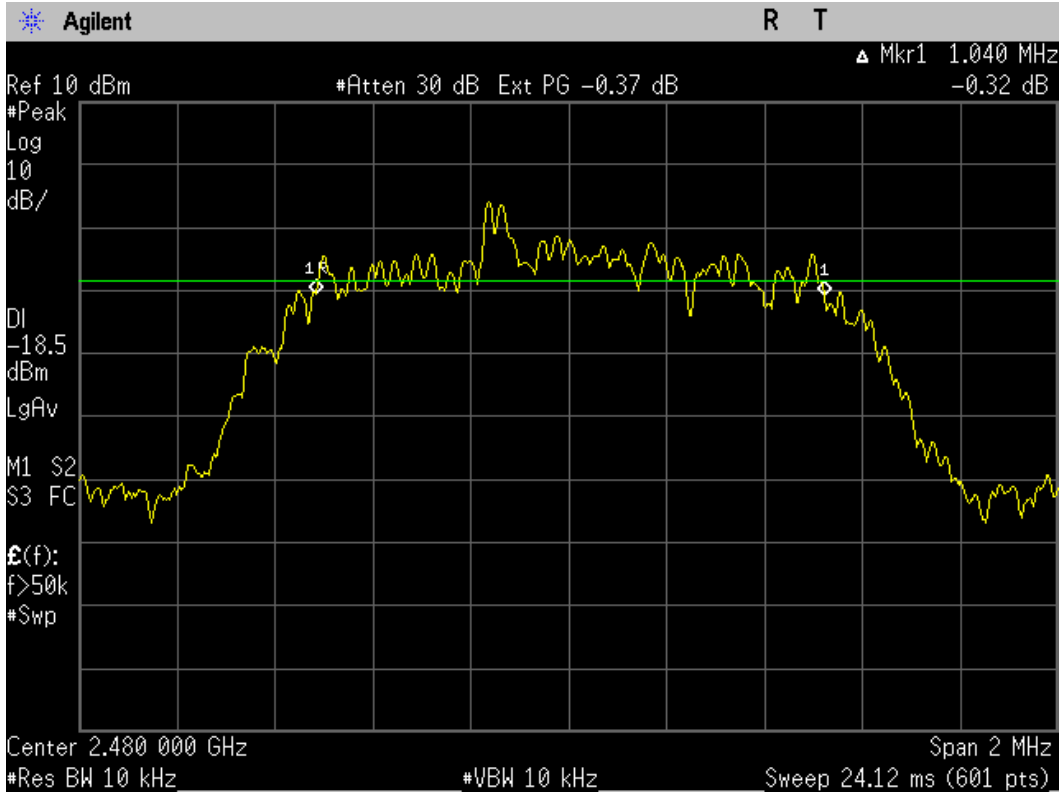
Figure 6-3c: 20dB Bandwidth EDR D8PSK, Channel 78.
