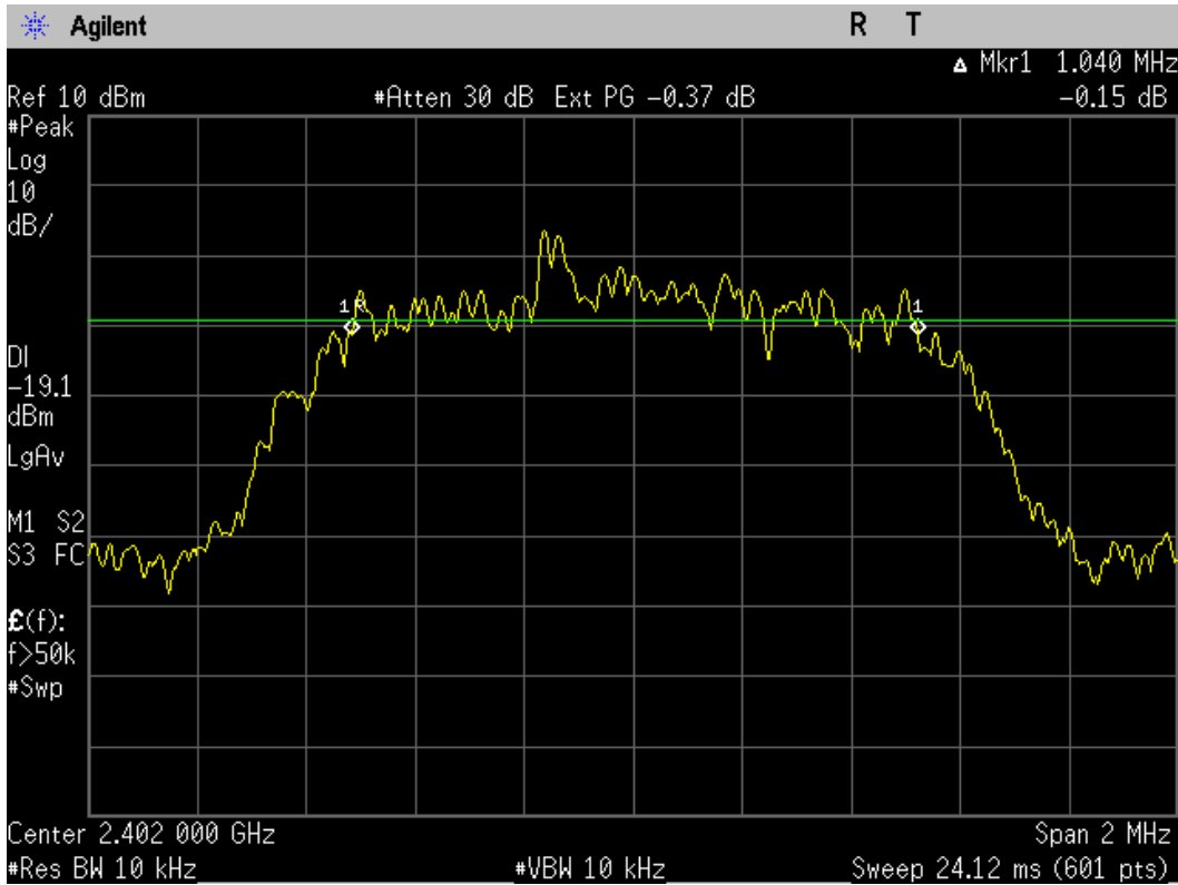
Figure 6-1c: 20dB Bandwidth EDR D8PSK, Channel 0.
