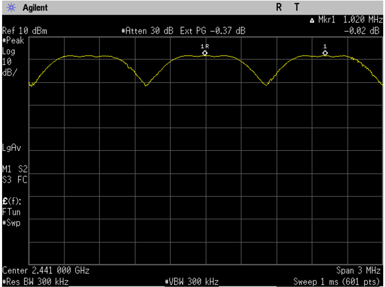
Figure 7: Carrier Frequency Separation between channels 38, 39 (mid-channel) & 40.
