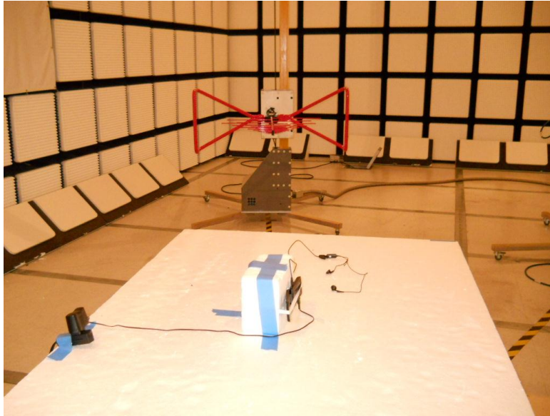
RADIATED BACK PHOTO 30-1000 MHZ
